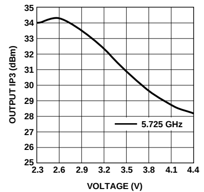
Figure 11. OIP3 vs. voltage at 5.725 GHz [4,5] .
