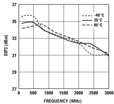
Figure 10. OIP3 vs Frequency (3V 60mA).
