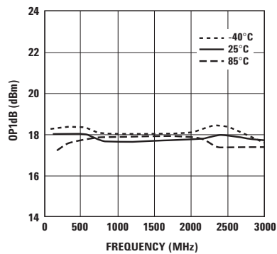
Figure 11. OP1dB vs. Frequency (3V 60 mA).
