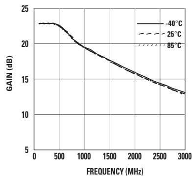
Figure 8. Gain vs. Frequency (3V 60 mA).
