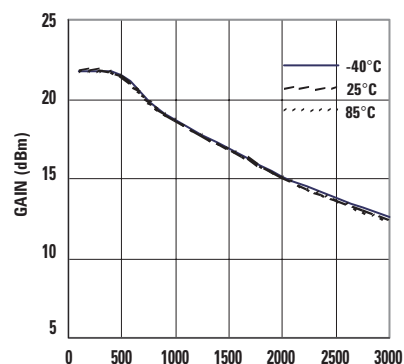
Figure 12. Gain vs. Frequency (3V 30 mA).
