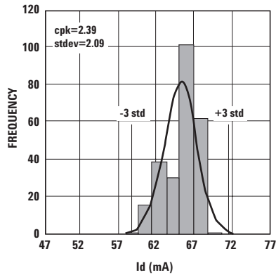
Figure 5. Id @ 3V. LSL=47, Nominal=62.0, USL=77.
