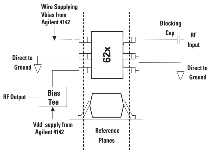
Figure 1b. A diagram showing the connection to the DUT during an S and Noise parameter measurement using an automated tuner system.
