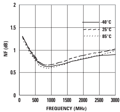
Figure 9. NF vs. Frequency (3V 60 mA).
