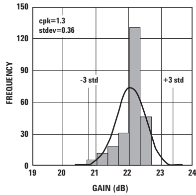
Figure 3. Gain @ 0.5 GHz 3V 60 mA. USL=23.4, Nominal=22.0, LSL=20.4.
