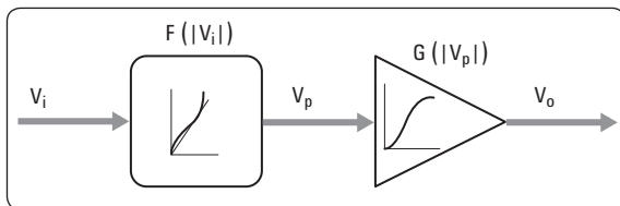
Figure 2. Predistortion applied to a non-linear power amplifier.
