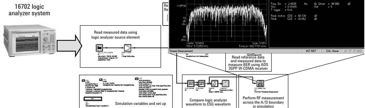
Figure 1. Post processing measured digital data with the 89600 VSA simulation software.
