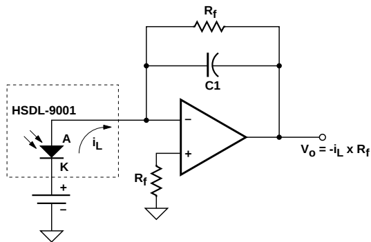
Figure 1. Typical application for HSDL-9001.
