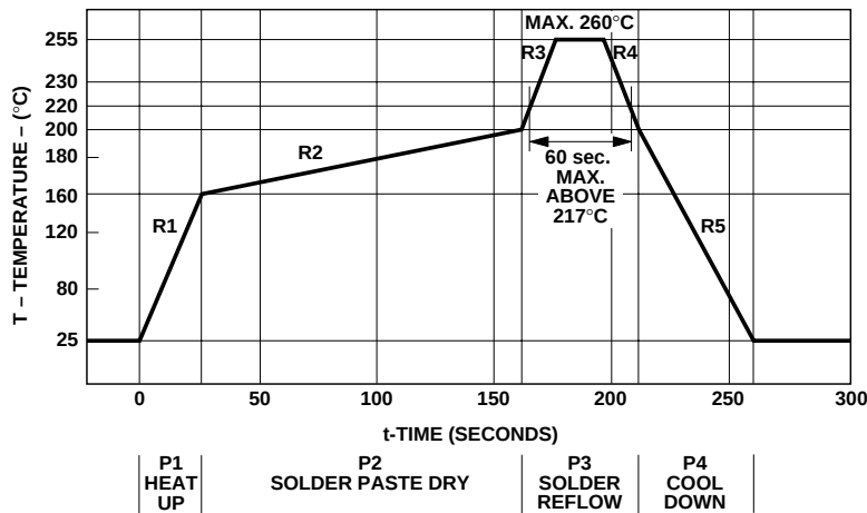
Figure 6. Reflow graph.
