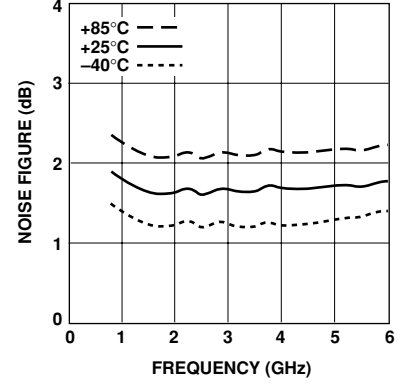
Figure 3. Minimum Noise Figure vs. Frequency and Temperature.
