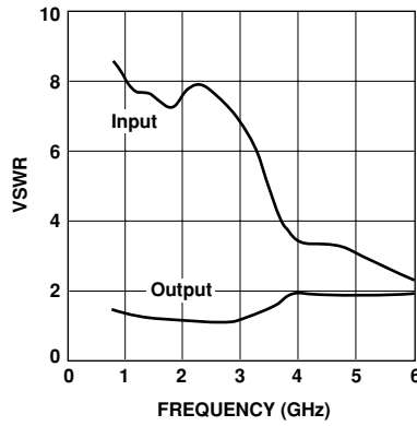
Figure 13. Input and Output VSWR vs. Frequency.
