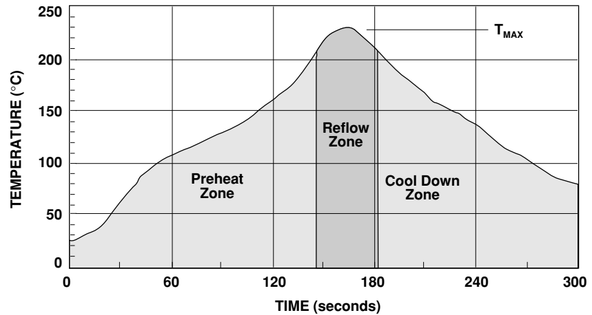
Figure 22. Surface Mount Assembly Profile.
