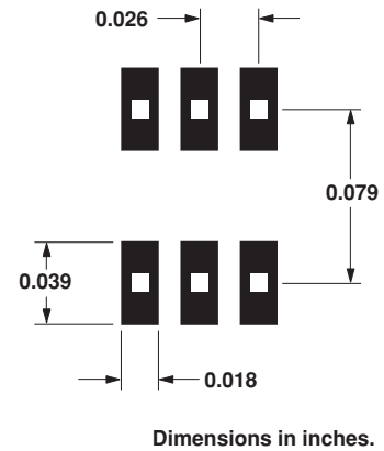
Figure 21. Recommended PCB Pad Layout for Agilent's SC70 6L/SOT-363 Products.
