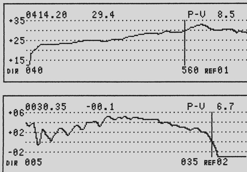
HP CaLan's Sweep/Ingress Analyzer provides displays of your forward (top) and return path.
