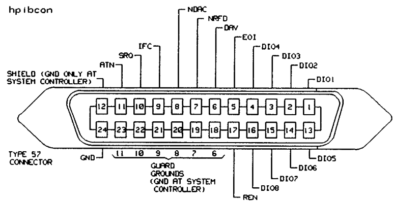
FIGURE C-4 HP-IB CONNECTOR
