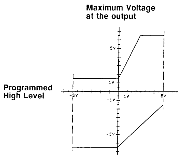
FIGURE 5-1. OUTPUT VOLTAGE WINDOW
