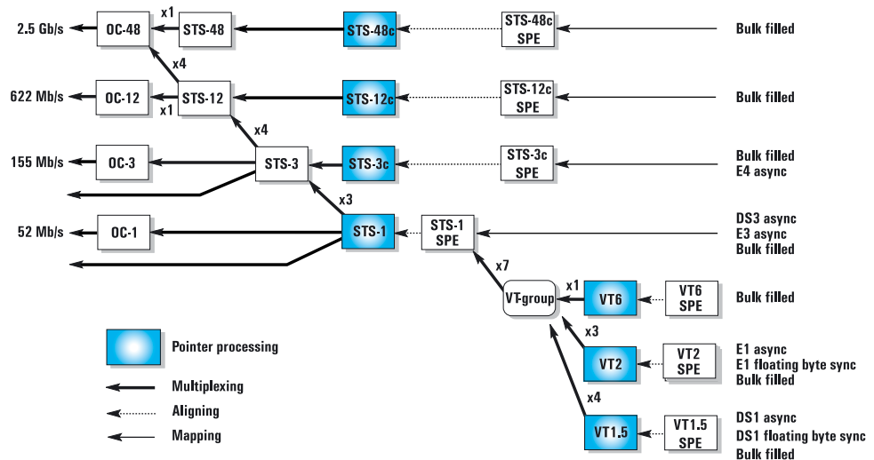
Figure 2: Bellcore GR-253 mapping structure (SONET payload mapping)
