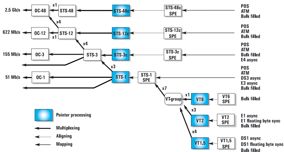
Figure 1: ITU-T G.707 mapping structure (SDH payload mapping)
