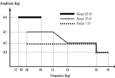
PDH/T-carrier generated jitter amplitude versus modulation frequency:
