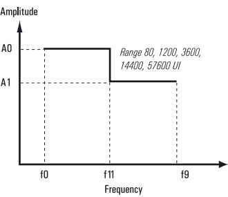
Generated wander amplitude versus modulation frequency:
