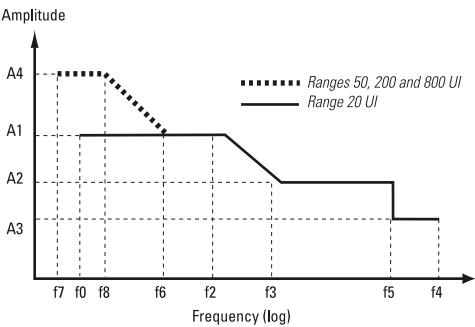
SDH/SONET generated jitter amplitude versus modulation frequency:
