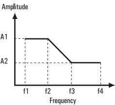
Bellcore GR-499 jitter amplitude versus modulation frequency:
