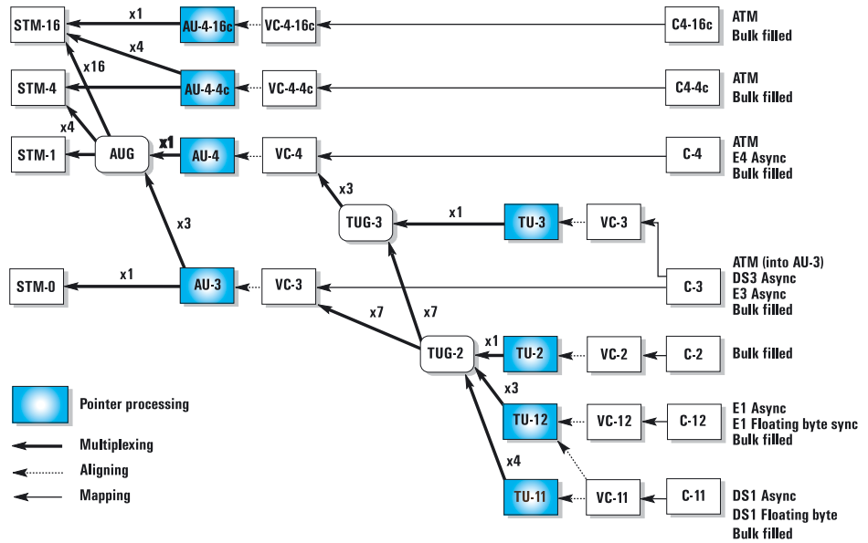
Figure 1: ITU-T G.707 mapping structure (SDH payload mapping)
