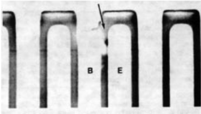
Figure 1. Bipolar Transistor with electrostatic discharge damage (2.5KX)
