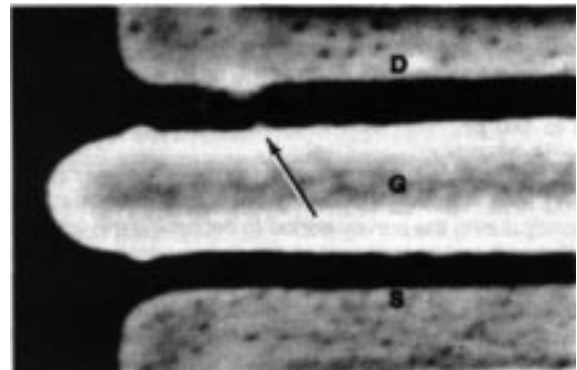
Figure 3. T-Gate Channel with Electrostatic Damage (5.8KX)
