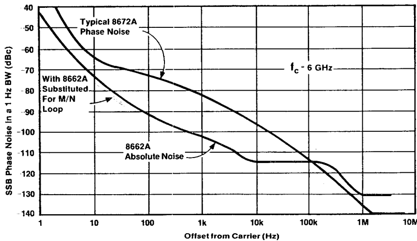
Figure 12.4. Effect of 8662A substitution on 8672A phase noise at 6 GHz.
