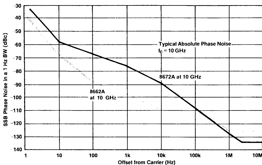
Figure 7.1. Phase noise comparison of 8662A and 8672A.
