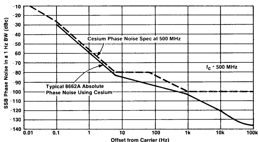
Figure 4.3. Effect of cesium on 8662A absolute noise.
