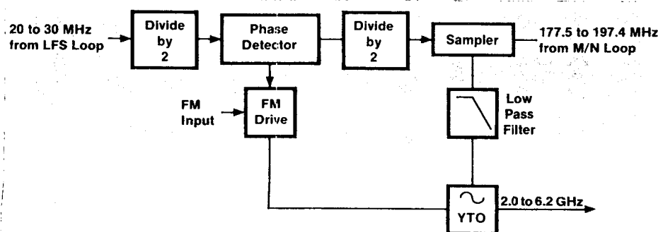
Figure 12.2. 8672A YTO loop.
