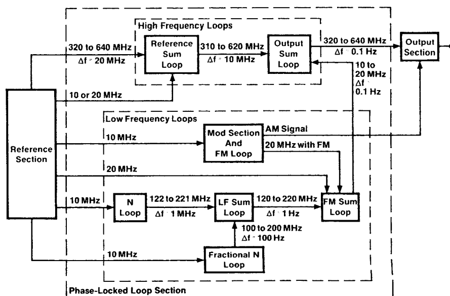
Figure 3.1. 8662A block diagram.
