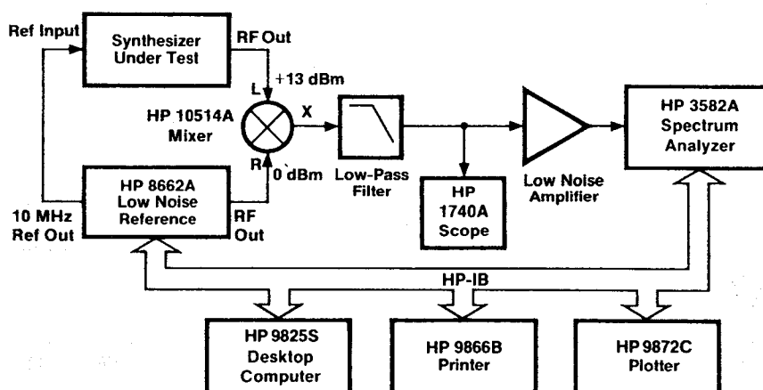
Figure 6.6. Automated system for phase noise measurement.
