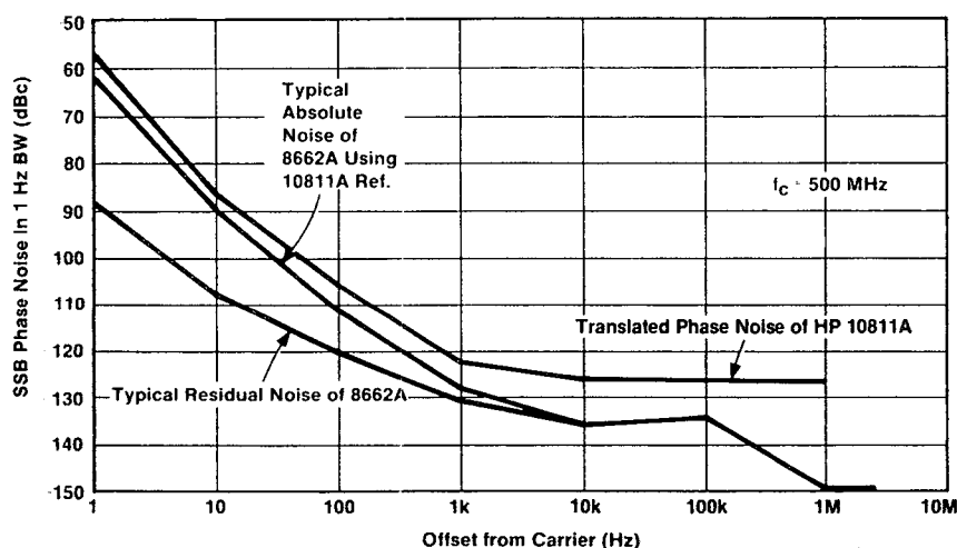
Figure 4.1. Comparison of 8662A noise vs. noise of internal reference.
