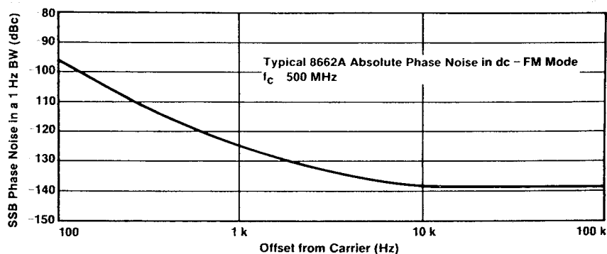
Figure 6.5. Typical 8662A absolute phase noise in dc-FM mode.
