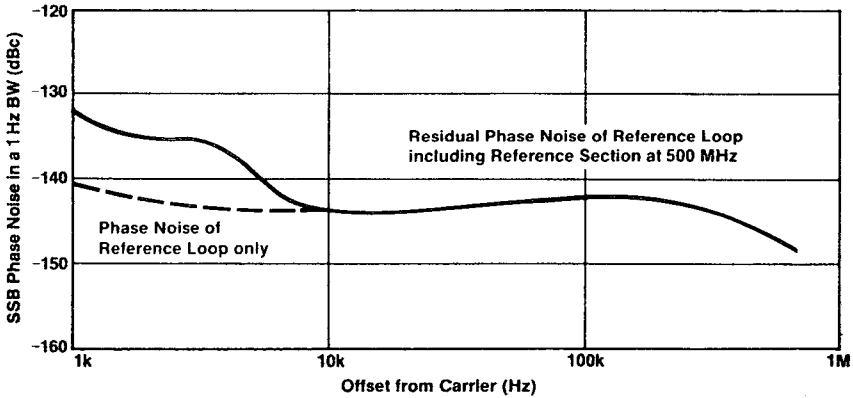
Figure 3.4. Typical phase noise of 8662A reference loop.
