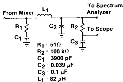
Figure 6.2. Low pass filter for two-source measurement.
