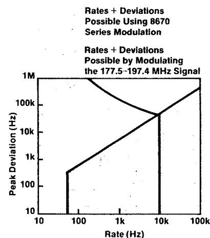
Figure 12.6. Increased FM performance with 8662A substitution.
