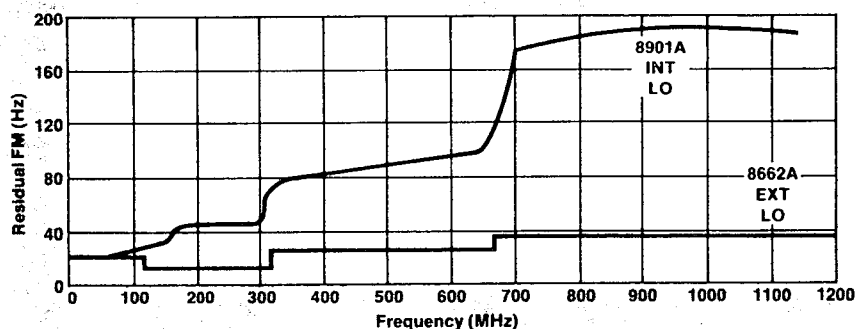
Figure 9.2. 8901A typical residual FM with no filtering.
