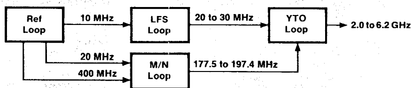
Figure 12.1. HP 8672A phase-lock loops.
