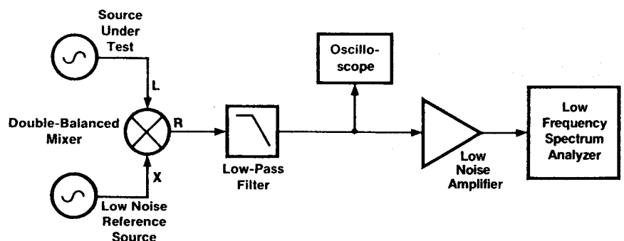
Figure 5.1. Basic two-source phase noise measurement set-up.
