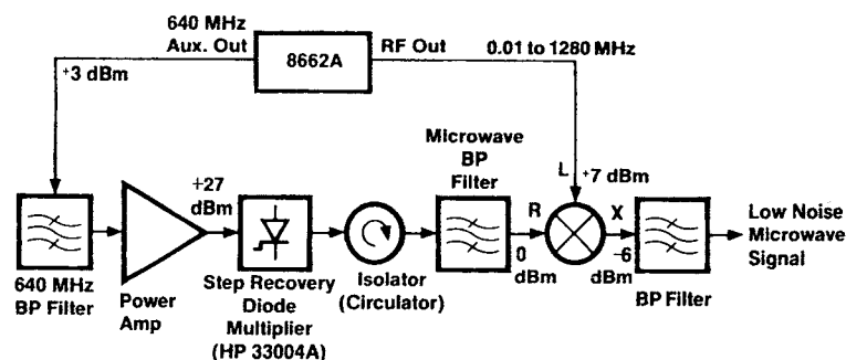
Figure 7.4. Low phase noise multiplication scheme for microwave signal generation.
