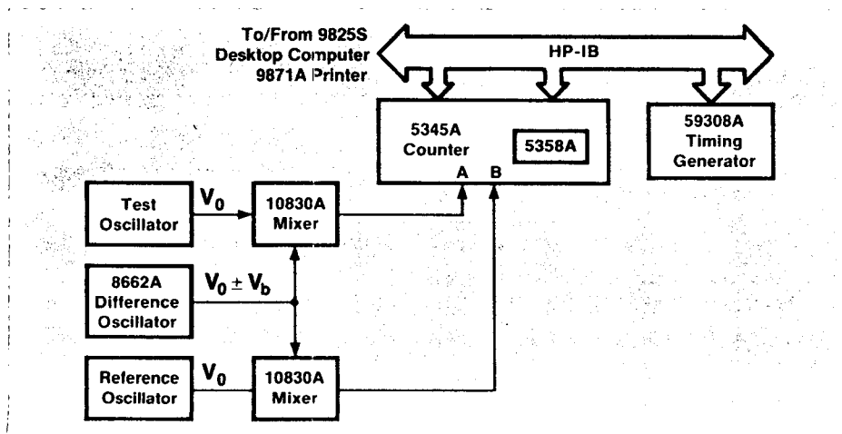
Figure 11.1. Dual mixer time difference set-up (HP 5390A Opt. 010).
