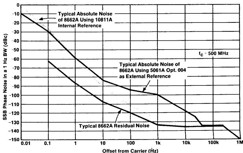
Figure 4.4. 8662A absolute noise comparison.
