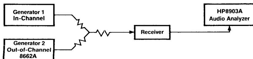
Figure 8.1. Receiver adjacent channel selectivity measurement.
