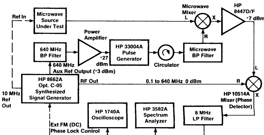
Figure 7.5. Microwave phase noise measurement using HP 8662A.
