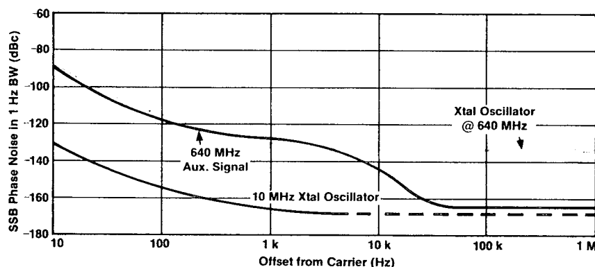
Figure 7.3. Phase noise of 640 MHz reference signal.
