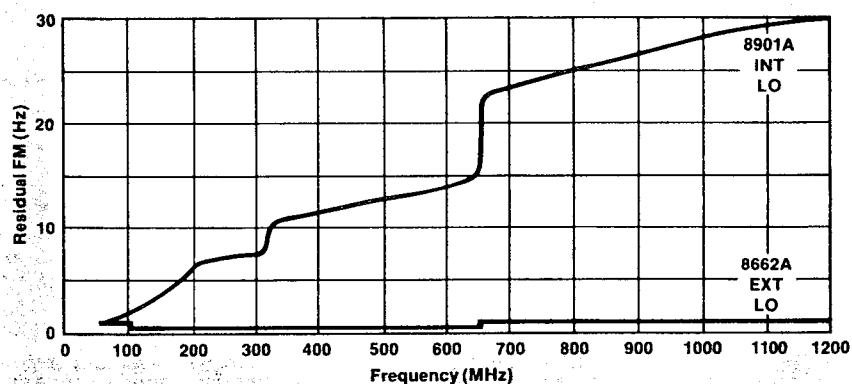
Figure 9.3. 8901A typical residual FM with 15 kHz LPF.
