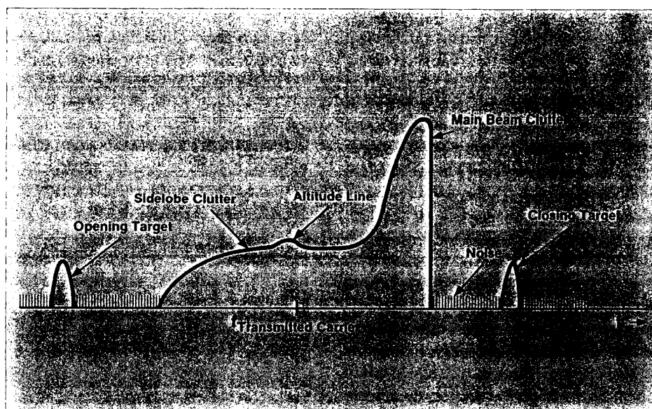
Figure 2.3. Typical return spectrum for airborne doppler radar.
