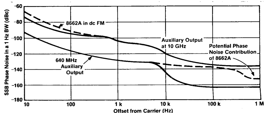
Figure 7.6. System absolute noise performance.
