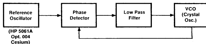
Figure 4.6. Narrowband phase-lock loop for two-reference system.
