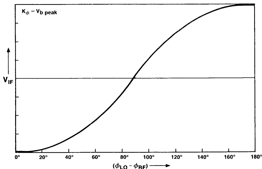
Figure 5.2. Typical double-balanced mixer phase detector characteristic.
