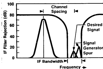
Figure 8.3. Signal generator spurious in adjacent channel test.
