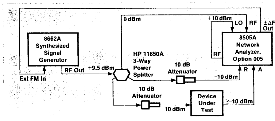
Figure 10.1. 8505A phase-lock test set-up with 8662A.
