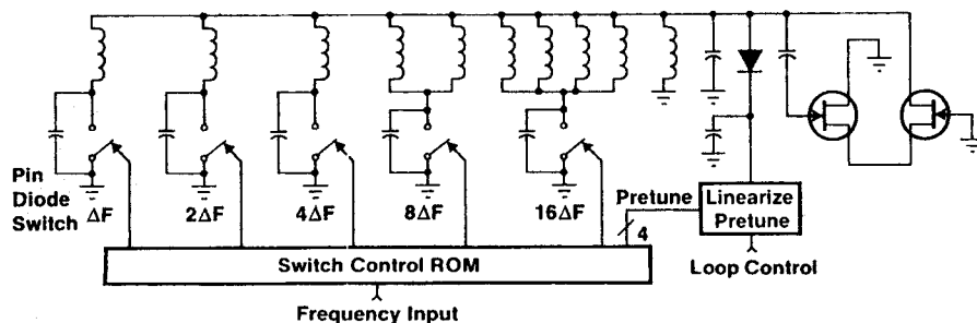
Figure 3.2. 320 to 640 MHz switched reactance oscillator.
