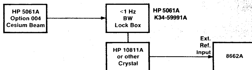
Figure 4.5. Using two references for optimal 8662A phase noise.
