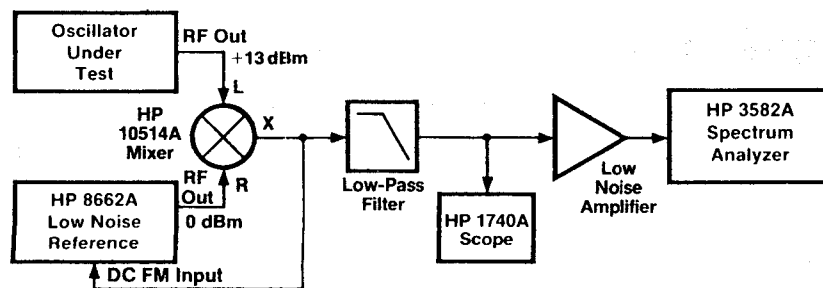
Figure 6.4. Phase-locked two source phase noise measurement.
