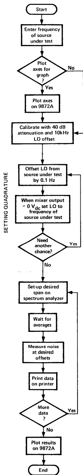
Figure 6.8. Flowchart for phase noise measurement.
