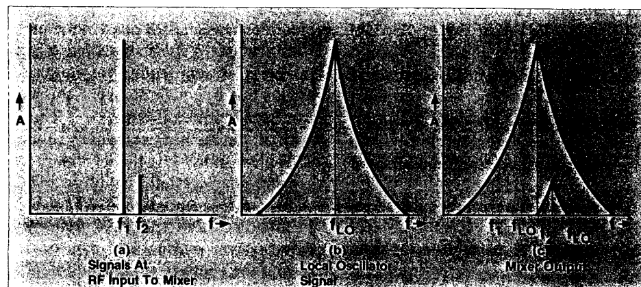
Figure 2.2. Effect of L.O. phase noise in mixer application.
