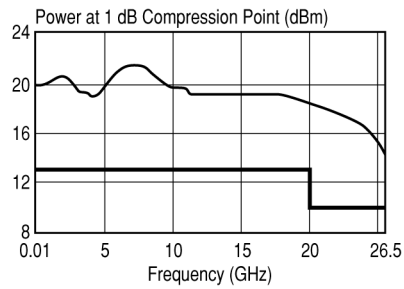
83006A Amplifier
