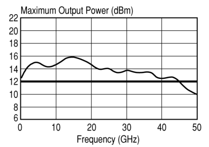
83051A Amplifier
