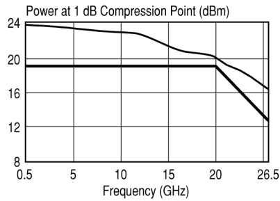
83017A Amplifier
