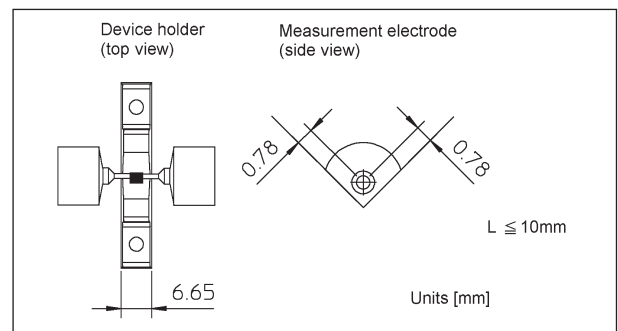
Electrode dimensions
