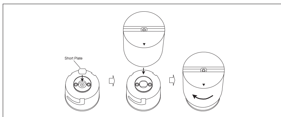
Short Compensation
