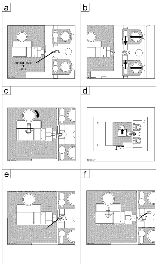
Open/Short compensation
