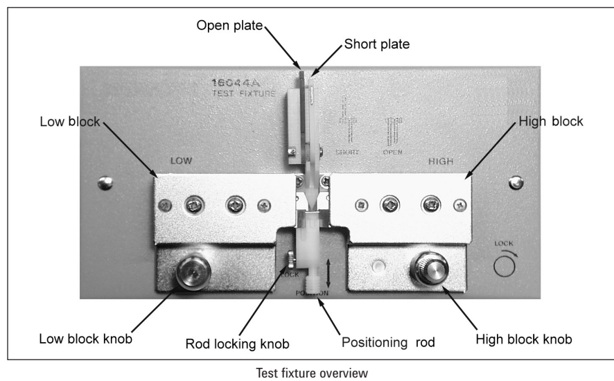
Test fixture overview
