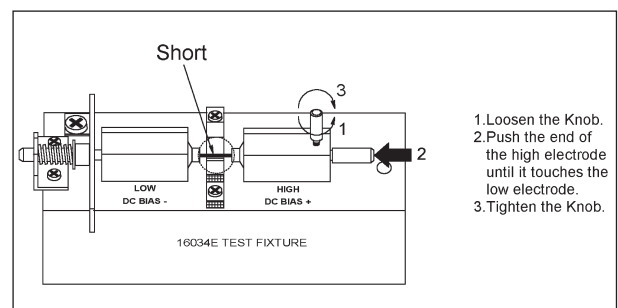
Short compensation
