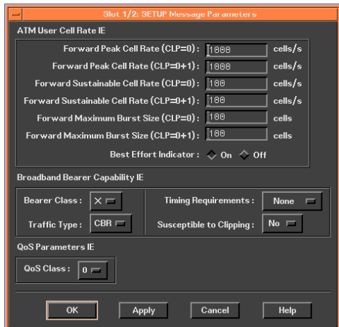
Screen 1: Signalling load test system needs to give the user control over a minimum number of elements of the SETUP message.
