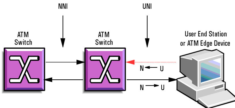
Figure 1: User-to-Network direction ATM switches which implement the signalling protocols at the User-Network Interface (UNI).
