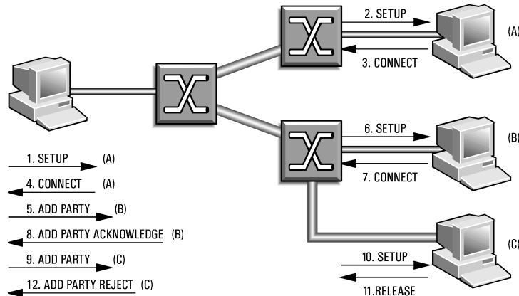
Figure 10: A P-MP call is initiated by one user (called the root) making a normal call to another user, (called a leaf node).
