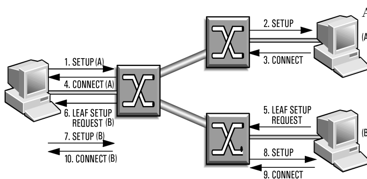
Figure 12: In a root LIJ, leaves join the call by sending a LEAF SETUP REQUEST to the network.
