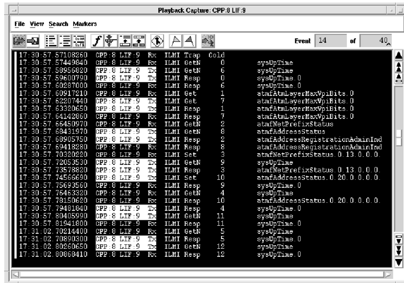
Figure 7: A captured ILMI address registration exchange from a BSTS shows data transmitted (Tx) from the analyzer (the user) and received from the network (Rx).
