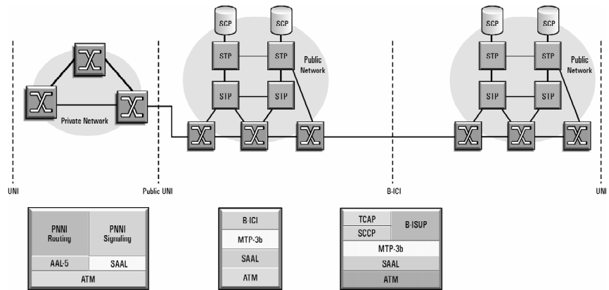
Figure 3: A complete protocol stack is used within, and between networks.
