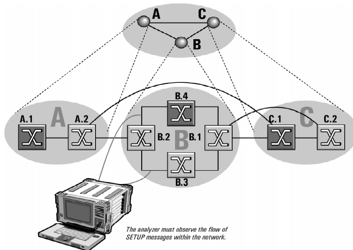
Figure 15: If monitor points are established at B.2/B.3 and B.2/B.4, the crankback can be observed.
