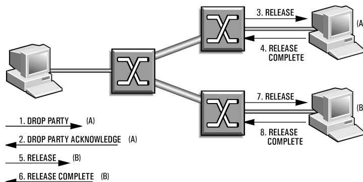
Figure 11: At the end of the P-MP, the root can remove leaves with the DROP PARTY message, or releases the entire call by sending a RELEASE message to the network.
