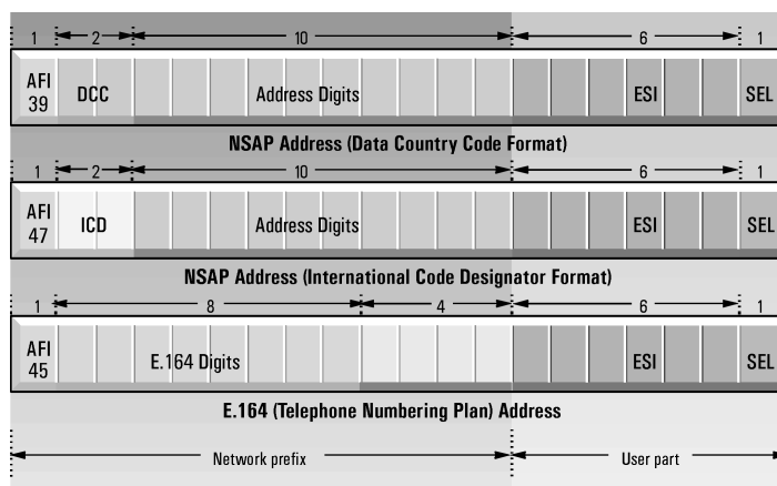
Figure 6: Each ATM address consists of three basic parts – the network prefix, the end system identifier, and a selector.
