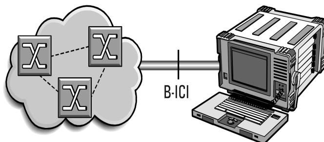
Figure 18: To generate potential non-conforming service requests into a network, an analyzer is connected.
