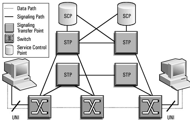
Figure 4: An SS7 network with a complex signalling network involving many nodes and multiple networks.
