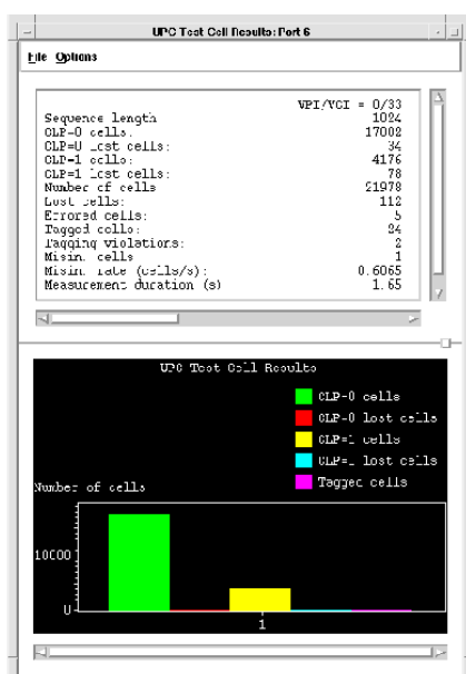
Figure 20: Results of a GCRA test on the Agilent BSTS.
