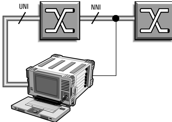
Figure 17: Configuring a protocol analyzer: at the UNI, the tester can either be used to emulate the calling party, or it can be used to monitor the signalling at the UNI. At the NNI, the analyzer can also be used to emulate a switch, or to monitor the link between two switches.
