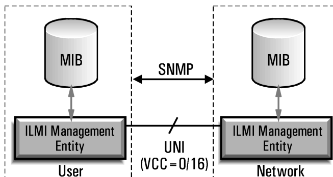
Figure 5: The user and network both contain databases, known as Management Information Bases, which store a variety of information related to the link between the two endpoints.
