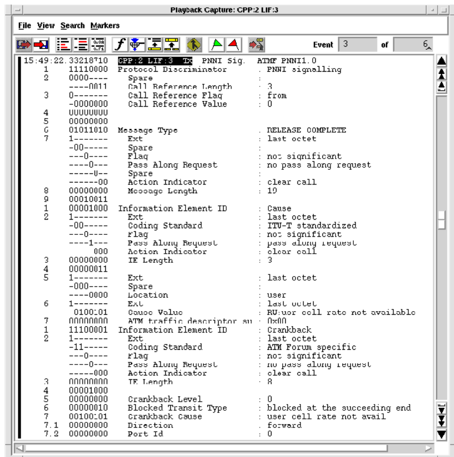
Figure 16: RELEASE COMPLETE message decoded on a Agilent Broadband Series Test System.
