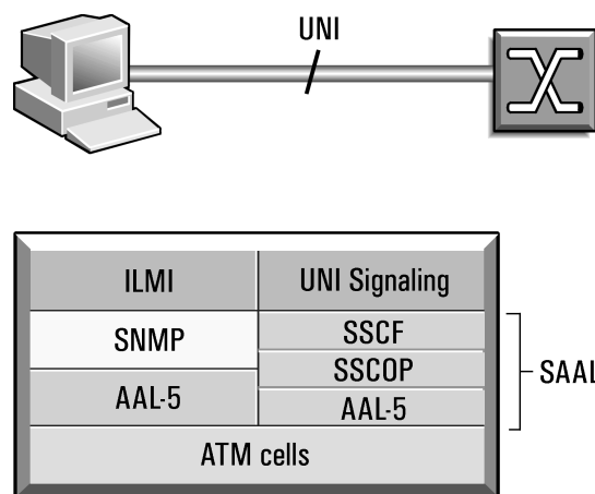
Figure 2: Protocols at the User-Network Interface.
