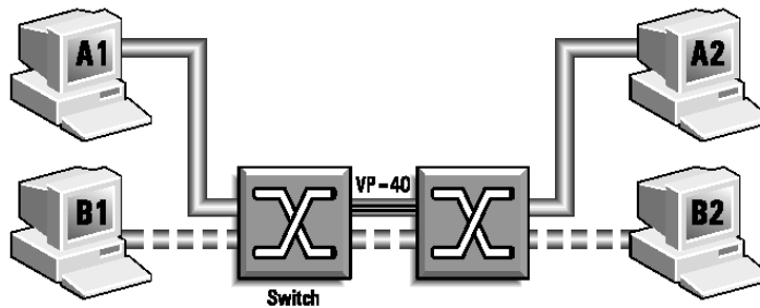
Figure 2: Simplified network diagram showing two switches and four end stations
