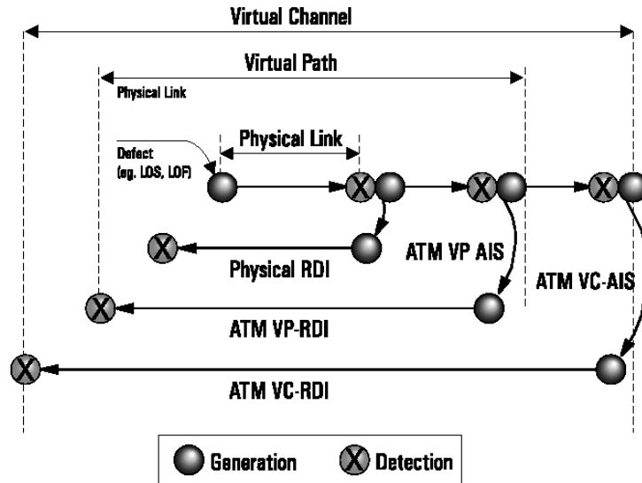
Figure 11: A physical layer alarm eventually causes both path (F4) and channel (F5) OAM RDI's
