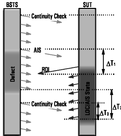
Figure 13: Stops generating AIS or RDI cells after receiving the first continuity check OAM cell
