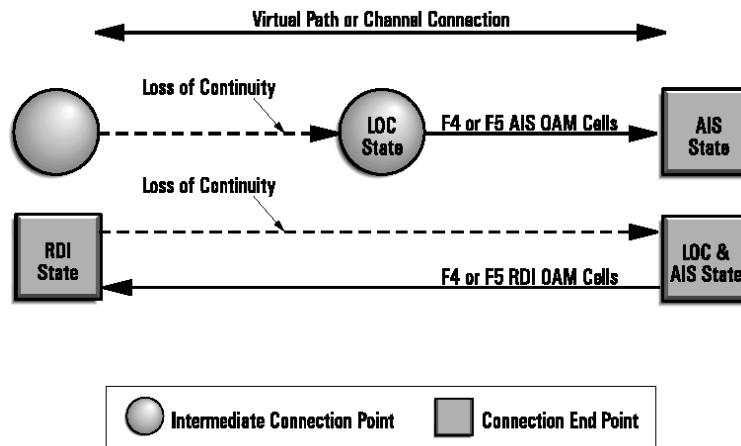
Figure 12: AIS OAM cells should be transmitted on the downstream connection to alert the connection end point
