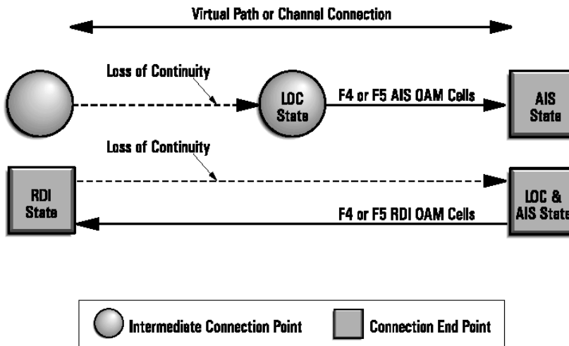
Figure 6: Reporting defects using AIS and RDI cells
