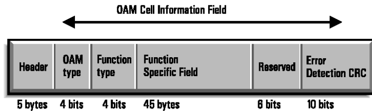
Figure 3: General format of an OAM cell
