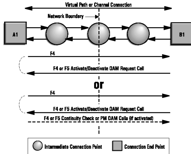
Figure 18: A continuity check function
