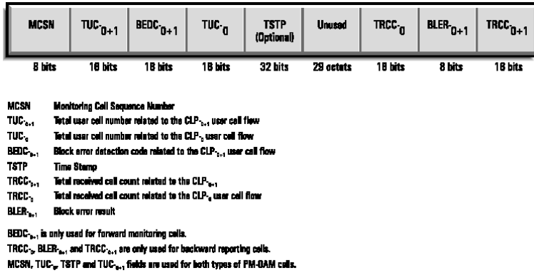
Figure 9: Two kinds of OAM performance management cells are defined
