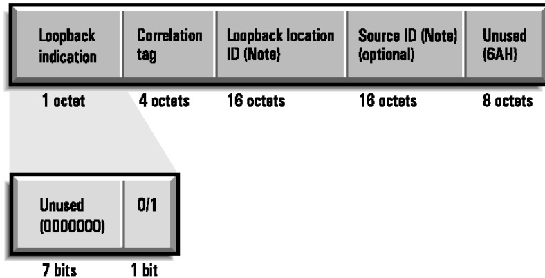
Figure 7: Loopback cells are used to determine connectivity at specific points in a network. Note: Values (except for default all 1's) are not subject to standardization and encoding of non-default values is optional.
