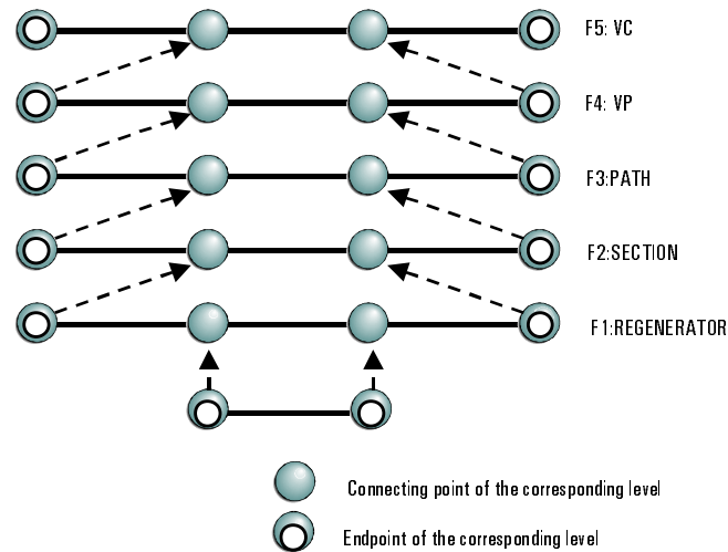
Figure 1: ITU-T considers an ATM network to consist of five flow level
