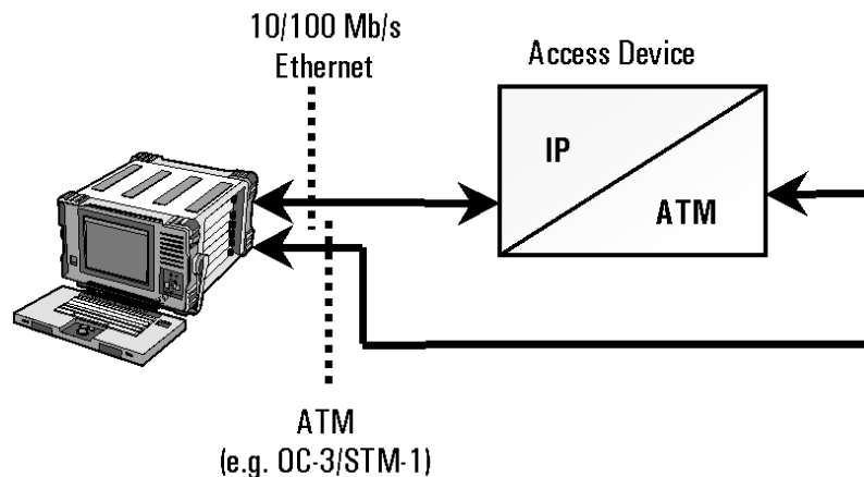
Test configuration #3: Test equipment with Ethernet and ATM ports connected to an interworking device.
