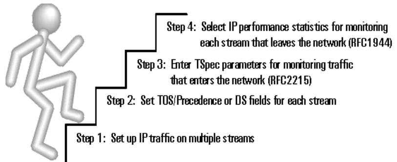
Test methodology for CoS contract verification in an IP network
