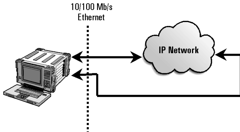
Test configuration #2: Dual-port 10/100 Mb/s Ethernet tester connected to an IP network: This configuration can also be used to test ADSL modems that have Ethernet access ports.
