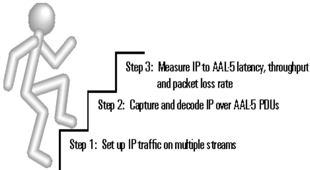
Test methodology for interworking testing of an IP/ATM access device
