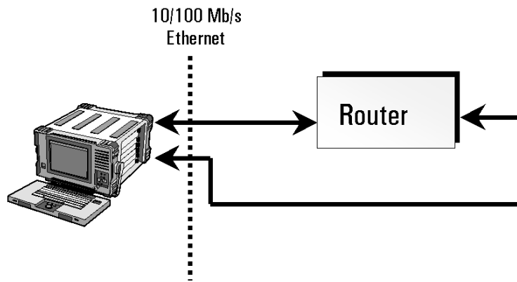
Test configuration #1: Dual-port 10/100 Mb/s Ethernet tester connected to a router.
