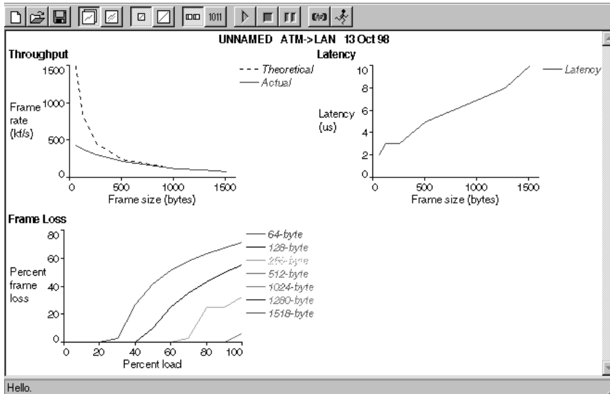
An example of how the results of your performance tests can be plotted graphically to discover performance trends.
