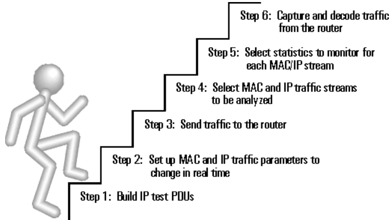
Test methodology for functional testing in order to find implementation problems at the MAC and IP layers.
