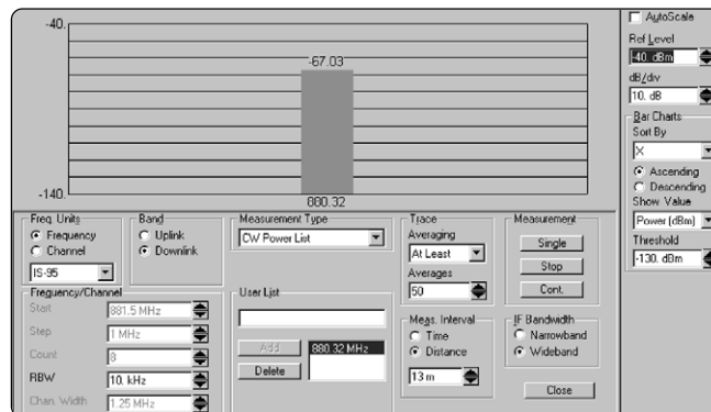
Figure 7. CW/channel power
