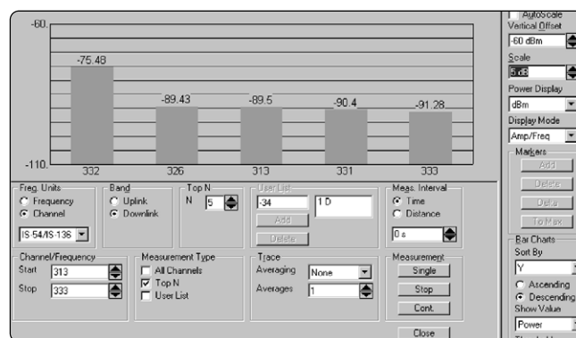
Figure 9. Channel analyzer
