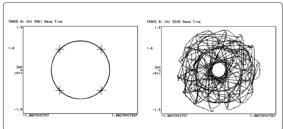
Figure 2. The GSM signal on the left has a constant power envelope, unlike the EDGE signal at right. The plot represents the carrier magnitude and phase at any given point in time. Since the carrier amplitude for GSM is constant, the carrier trajectory forms a perfect circle.
