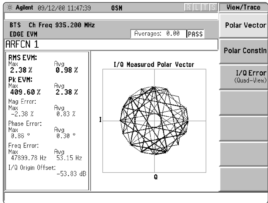
Figure 18. When ISI compensation is applied to an EDGE vector/constellation diagram at 1 point/symbol the confusing effects of ISI are eliminated and a useful constellation is produced without the distortion of zero-forcing or complimentary filters.
