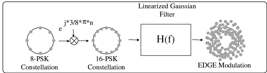
Figure 8. EDGE modulation begins with an 8-PSK constellation, which then undergoes 3\pi/8 rotation (similar to IS-136 \pi/4 rotation), and is then filtered using a linearized Gaussian filter before transmission.
