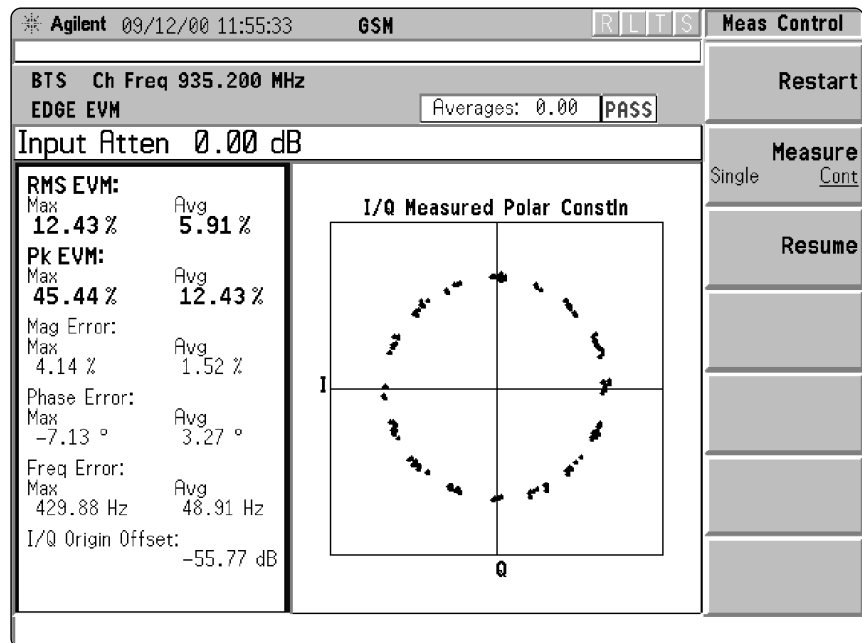
Figure 19. With ISI removed, this constellation diagram clearly shows the presence of undesirable phase modulation or phase noise.
