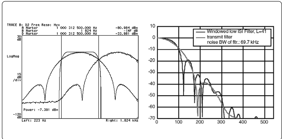
Figure 15. The effects of windowing on the RC filter are clearly visible in these plots. The frequency response of the original filter is shown at left while the windowed version is shown on the right (the darker trace). Note that the sidelobe structure introduced as a result of the windowing causes the response to follow the spectral shape of the EDGE signal.
