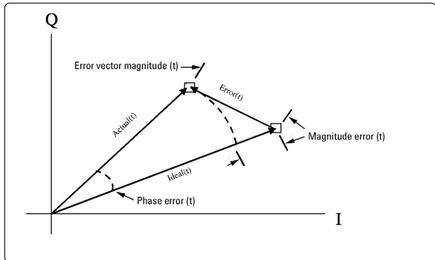
Figure 17. EVM and the error vector defined.
