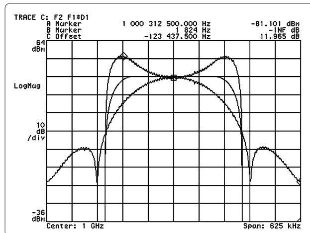
Figure 11. To satisfy the Nyquist criteria and provide a zero-ISI response (middle trace), a zero-forcing or complementary filter (upper-most trace) is applied to the transmitted signal (bottom-most trace).
