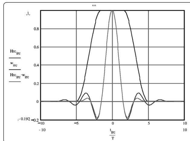
Figure 14. This plot shows the impulse response of the original raised-cosine filter, the windowing function (outer-most trace), and the resulting windowed raised-cosine filter (the more centered trace, closer to zero), which is the product of the first two. The plot reveals significant ringing in the original filter beyond the \pm five-symbol interval, while the impulse response of the new filter is zero outside this range.
