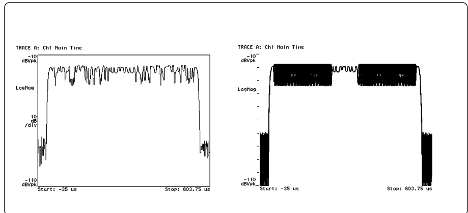
Figure 4. The power vs. time plot at left shows a single EDGE burst, while several hundred bursts are overlaid in the plot at right.
