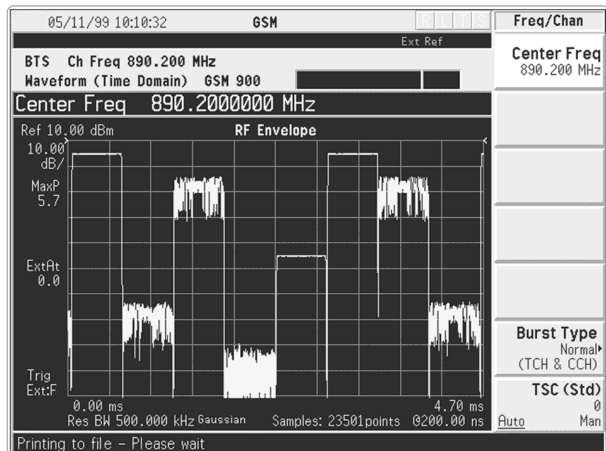
Figure 5. This PvT plot shows both EDGE and GSM bursts in a single frame (plus one empty slot). The signal is generated using two Agilent E4433B ESG series signal generators. One signal generator is used to produce the EDGE bursts at two different power levels. The other generates the GSM bursts, also at different power levels.
