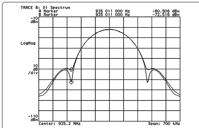
Figure 1. GSM and EDGE signals can typically be distinguished by inspecting the nulls at the edges of the main lobe. As seen in this plot, the EDGE spectrum (bottom trace) exhibits much deeper nulls.
