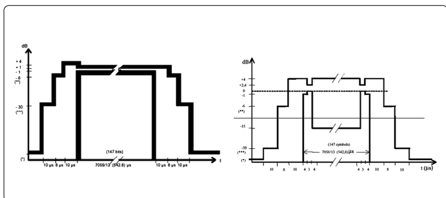
Figure 3. The EDGE signal's amplitude modulation component requires a different power-versus-time mask (right) for measurement than GSM (left).
