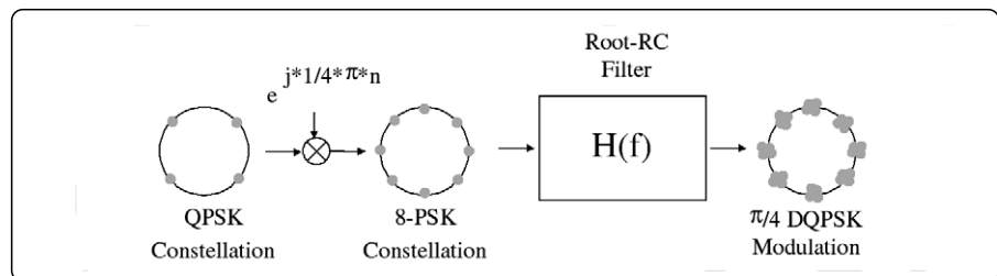
Figure 6. IS-136 TDMA-based systems use \pi/4 DQPSK modulation for transmitted signals.
