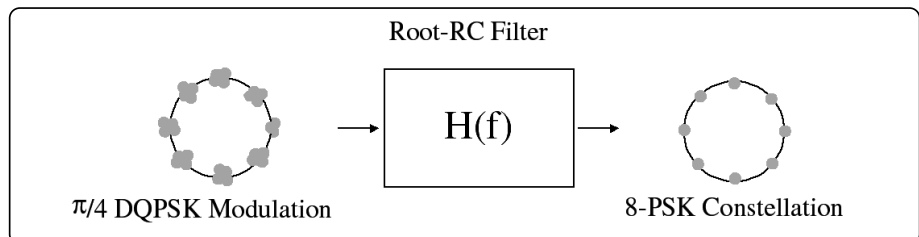
Figure 7. Once received and filtered, the quality of the \pi/4 DQPSK modulated signal is easily assessed by looking at the spread of points in the resulting 8-PSK constellation.
