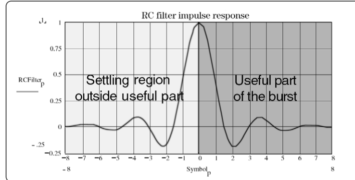
Figure 13. The first proposed 0.25 alpha, raised-cosine filter's impulse response has the potential to introduce errors into the useful part of the signal burst from the settling region, or even from adjacent time slots!
