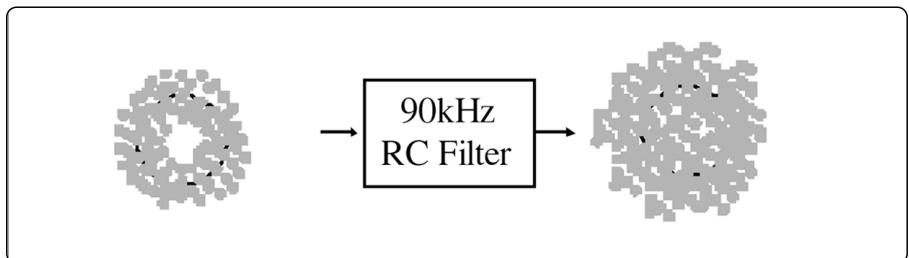
Figure 16. EDGE transmitted constellation, before and after filtering with the “windowed” 90 kHz RC filter.
