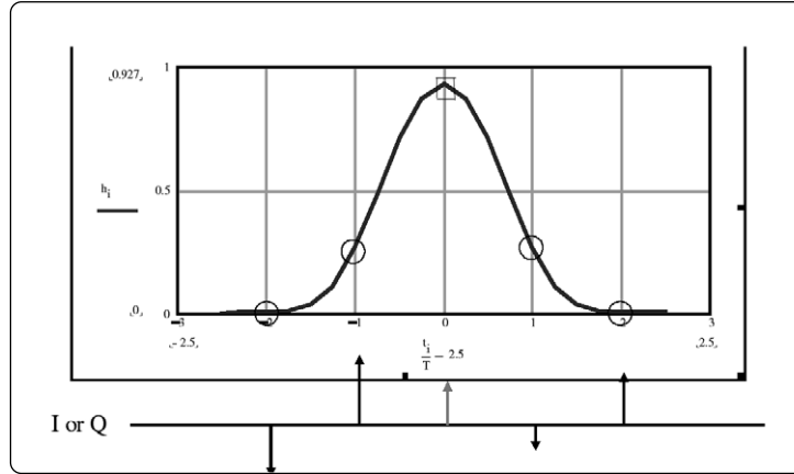
Figure 9. This is a plot of the impulse response of the linearized Gaussian filter. Note that the impulse response is wide enough (long enough in time) that each symbol point in the filtered constellation contains significant contribution from several symbols — the symbol of interest, plus the two symbols at either side.
