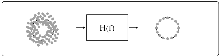
Figure 10. For measuring a received EDGE signal, it would seem that minimizing ISI (and possibly limiting the bandwidth) might be the goal of filtering. This could be accomplished by using a “zero-forcing” measurement filter as shown here.
