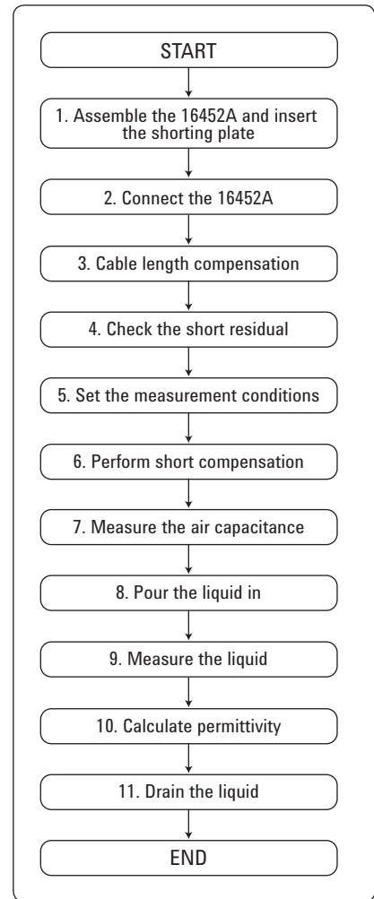
Figure 34. Measurement procedure flowchart for the 16452A
