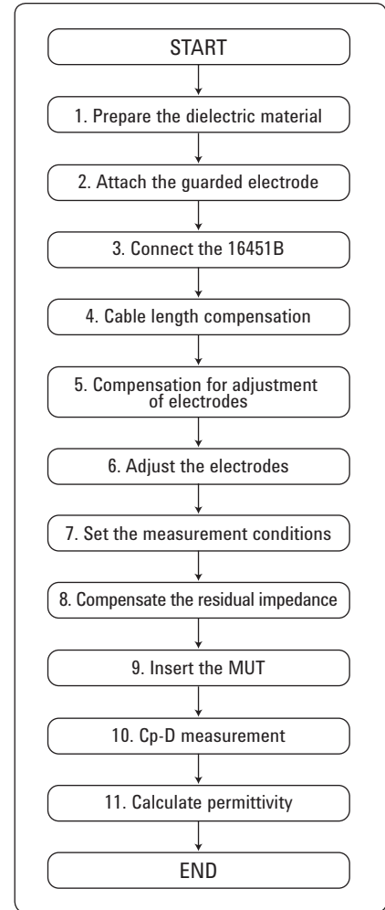
Figure 14. Measurement procedure flowchart for the 16451B
