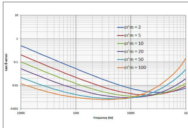
Figure 18. Loss tangent measurement accuracy (supplemental data)
