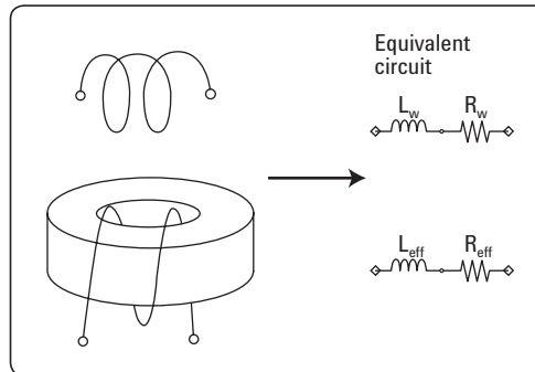
Figure 25. Method of measuring effective permeability
