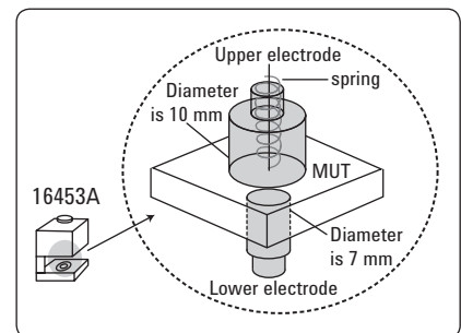
Figure 16. Structure of the 16453A
