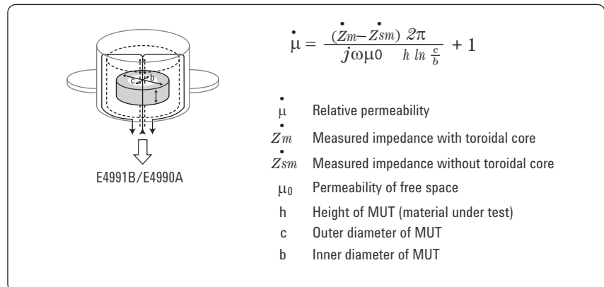
Figure 27. Structure of the 16454A and measurement concept
