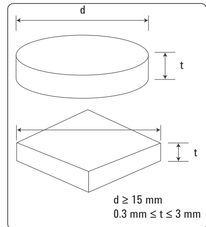
Figure 15. Applicable MUT size
