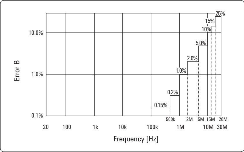
Figure 33. Relative measurement accuracy (supplemental data)
