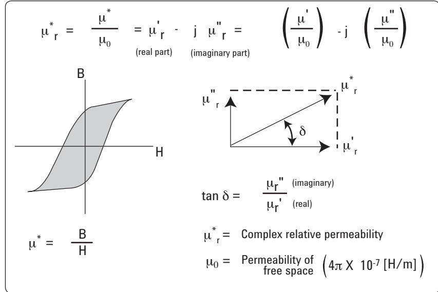
Figure 24. Definition of complex permeability ( \mu^* )
