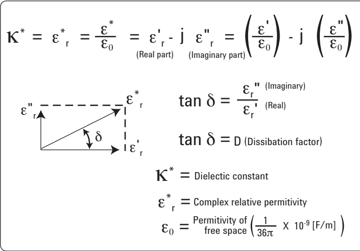
Figure 1. Definition of relative complex permittivity ( \epsilon_r^* )
