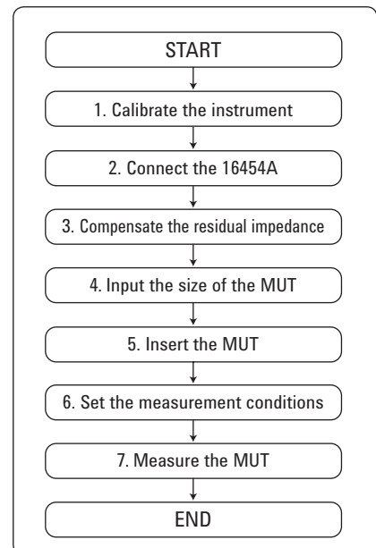
Figure 30. Measurement procedure flowchart for the 16454A
