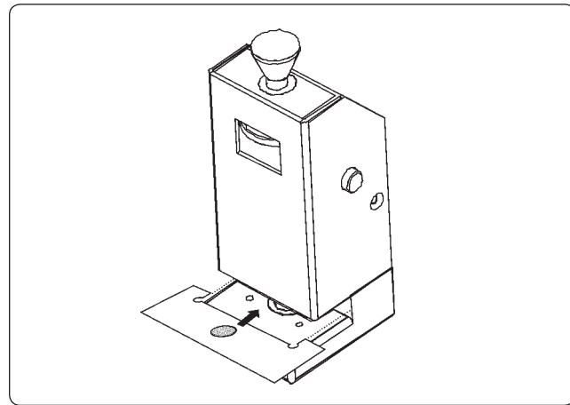
Figure 22. Positioning of the fabricated thin film on the MUT
