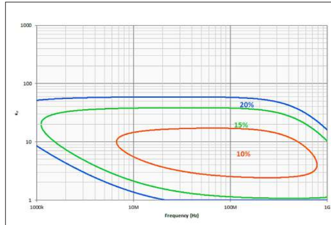
Figure 17. Permittivity measurement accuracy (supplemental data)
