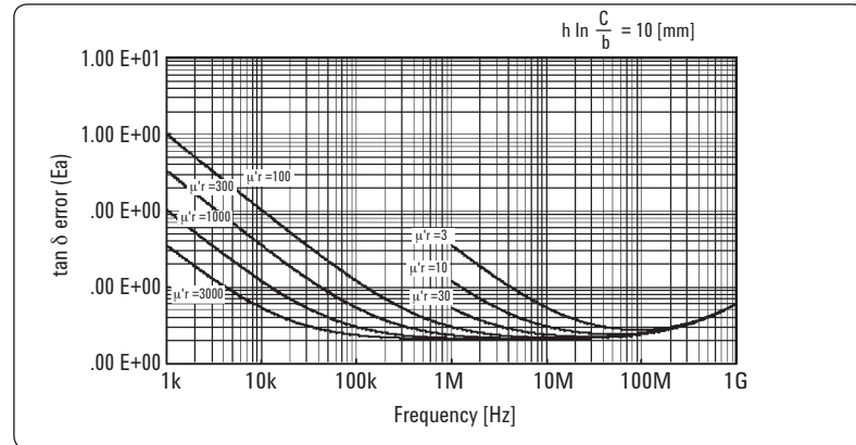
Figure 29. Loss tangent measurement accuracy (supplemental data)
