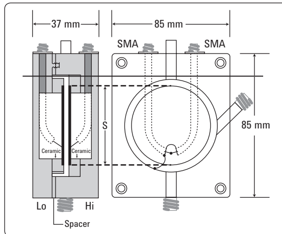
Figure 32. Structure of the 16452A
