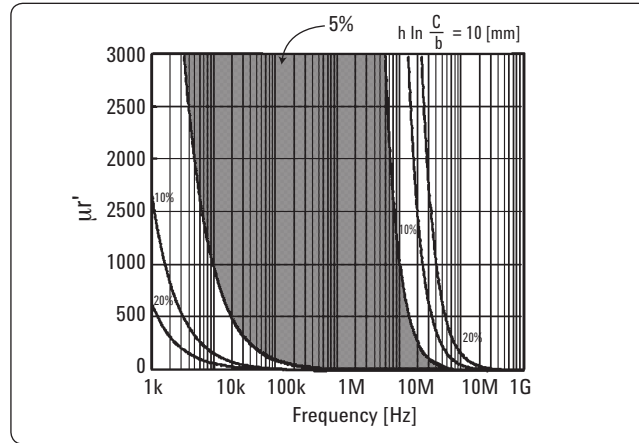
Figure 28. Permeability measurement accuracy (supplemental data)
