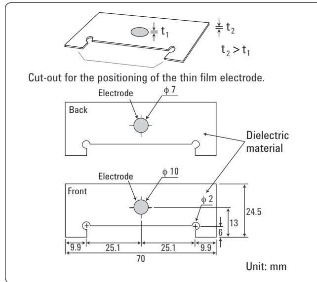
Figure 21. Fabricated thin film electrode's size
