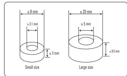
Figure 26. Applicable MUT size
