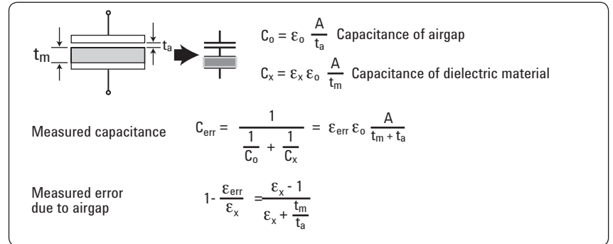
Figure 5. Airgap effects
