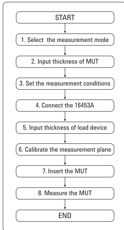
Figure 19. Measurement procedure flowchart for the 16453A
