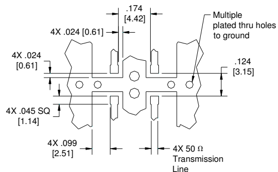
Dimensions are in Inches [Millimeters] 1P603S Mounting Footprint
