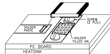
MOUNTING PROCEDURE
