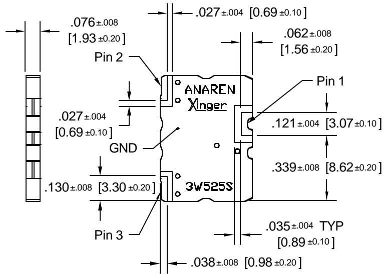
Bottom View (Far-side)
