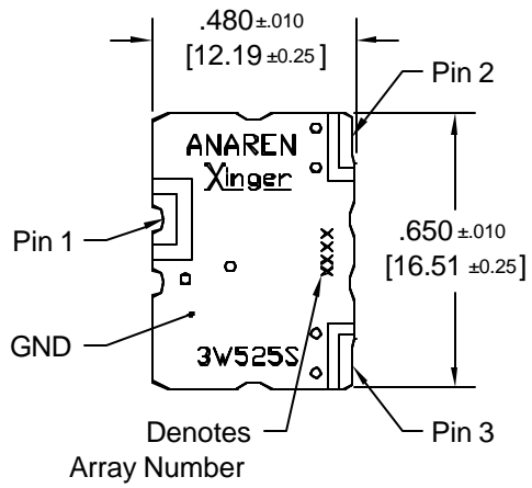
Top View (Near-side)
