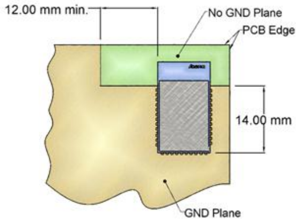
Figure 9 Mounting the module in a corner
