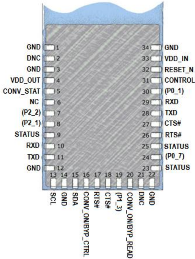
Figure 6 A2541R24x20 Module pin-out (viewed from top side)
