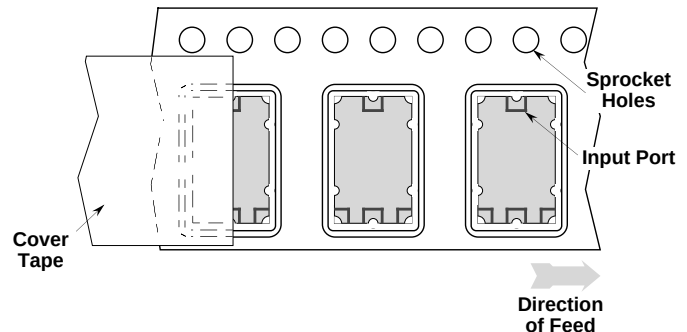
Tape & Reel Orientation of the 2 and 3 way Xinger Power Dividers
