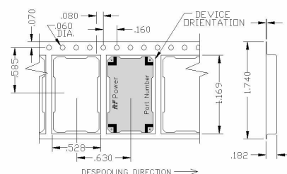
Case Style 'B' (1.00" x 0.50" Outline)
