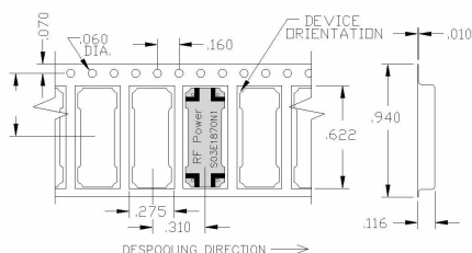
Case Style 'E' (0.56" x 0.20" Outline)
