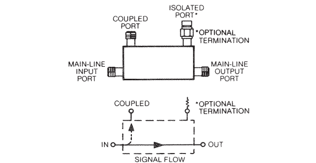
Figure 35 - H-Style Directional Coupler
