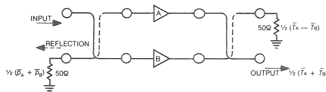
Figure 23 – Balanced Amplifier
