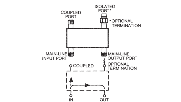
Figure 35 - H-Style Directional Coupler
