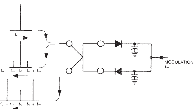
Figure 32 - 180° Balanced Modulator with Good Carrier Suppression, Poor VSWR
