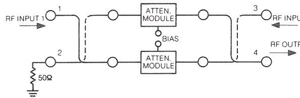
Figure 27 – Matched DPST Switch
