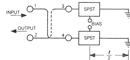
Figure 16 – Single-Bit Phase Shifter
