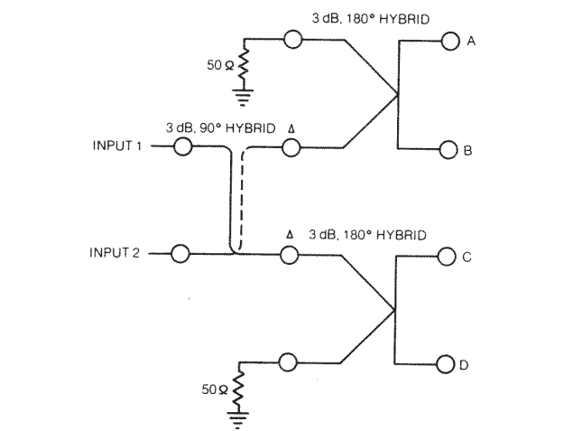
Figure 31 - Circular Polarization Network, LHC, RHC, Using Anaren Hybrids
