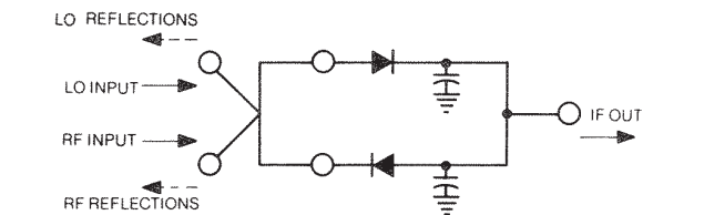
Figure 30 - 180° Balanced Mixer with Good LO/RF Isolation, Poor VSWR
