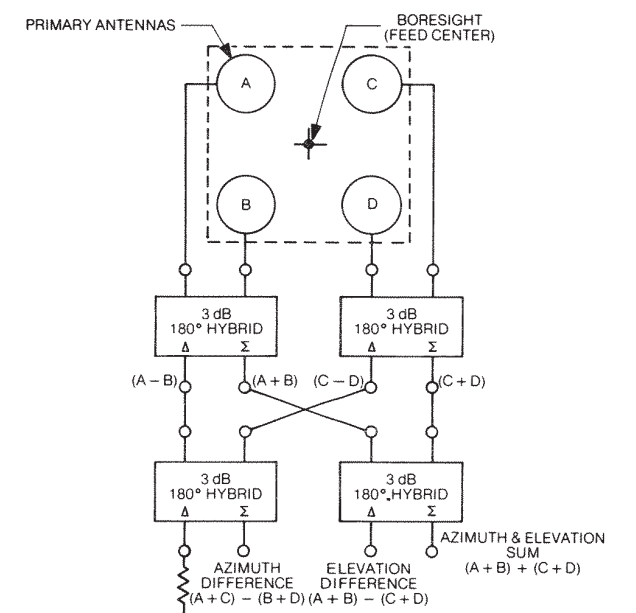
Figure 33 - Monopulse Tracking System
