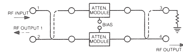
Figure 26 – Matched DPDT Switch
