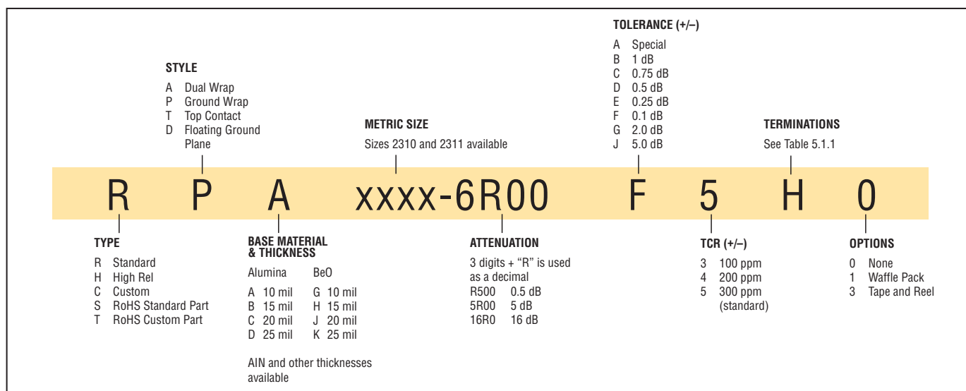
Figure 5.1.1: Part Numbering
