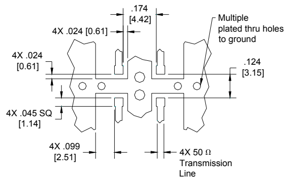
Dimensions are in Inches [Millimeters] JP503 Rev A Mounting Footprint
