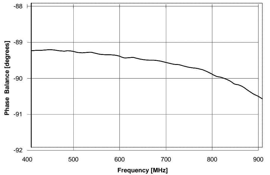
Phase Balance S03B665W3
