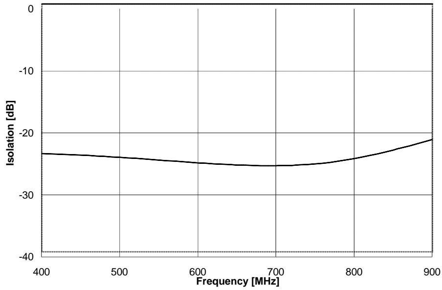
Isolation S03B665W3
