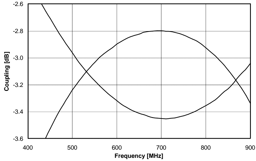
Coupling S03B665W3
