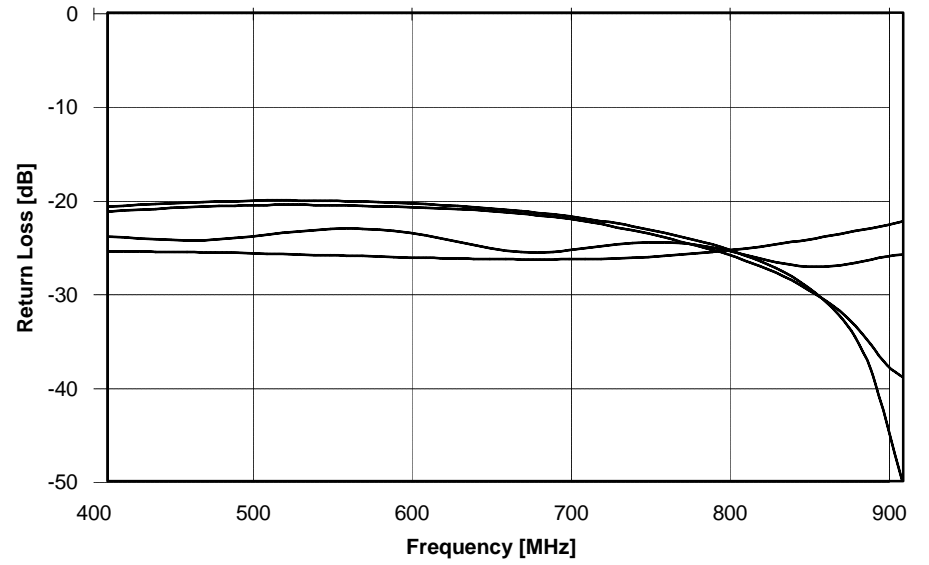
Return Loss S03B665W3
