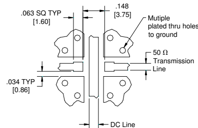
Dimensions are in Inches [Millimeters] X2A Rev A Mounting Footprint
