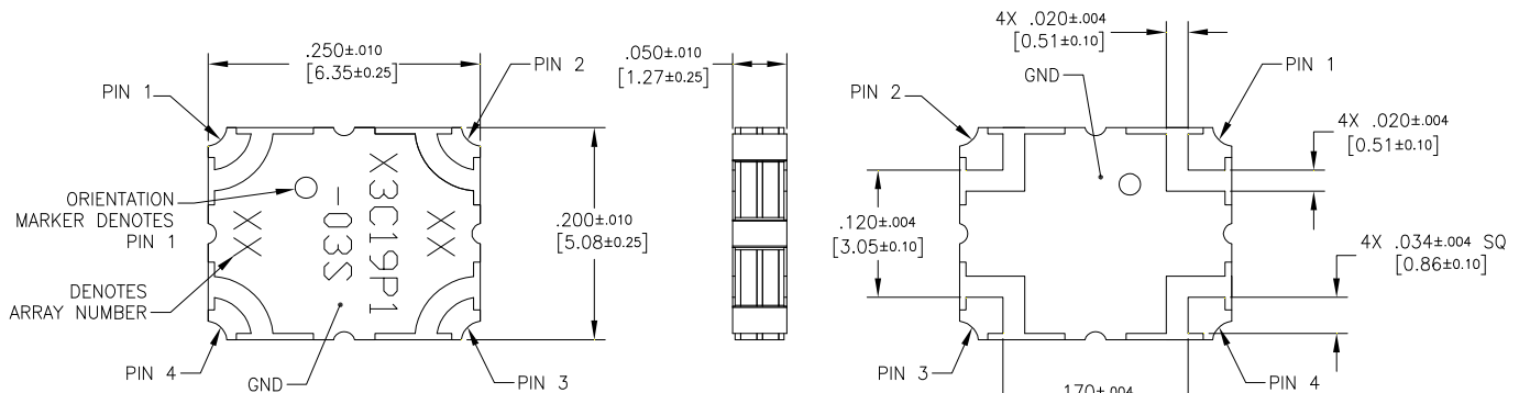
Dimensions are in Inches [Millimeters] X3C19P1-03S Mechanical Outline
