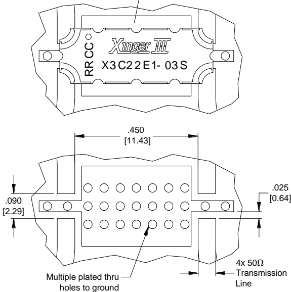
Dimensions Are in Inches [Millimeters] X3C22E1-03S Mounting Footprint
