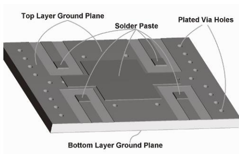
Figure 2: Solder Paste Application
