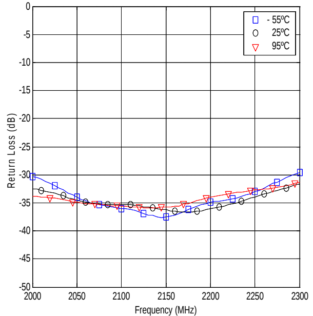
Return Loss for XC2100A-10 (Feeding Port 4)
