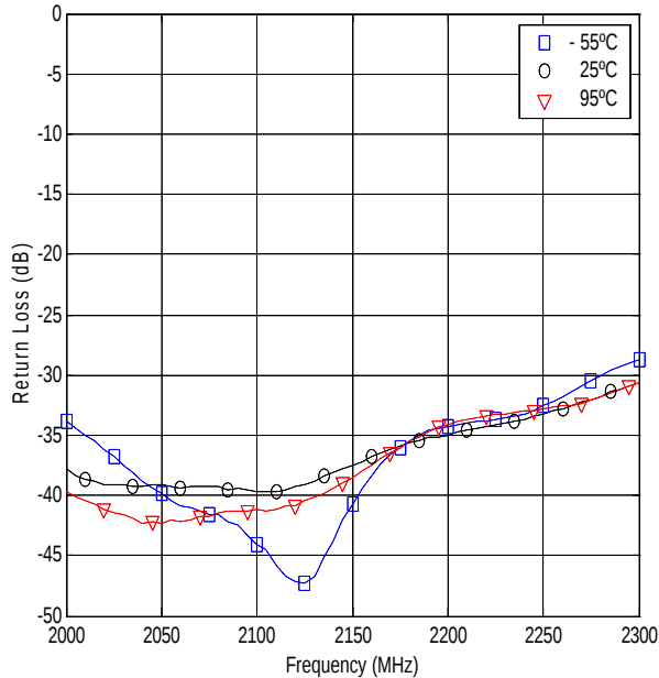
Return Loss for XC2100A-10 (Feeding Port 3)
