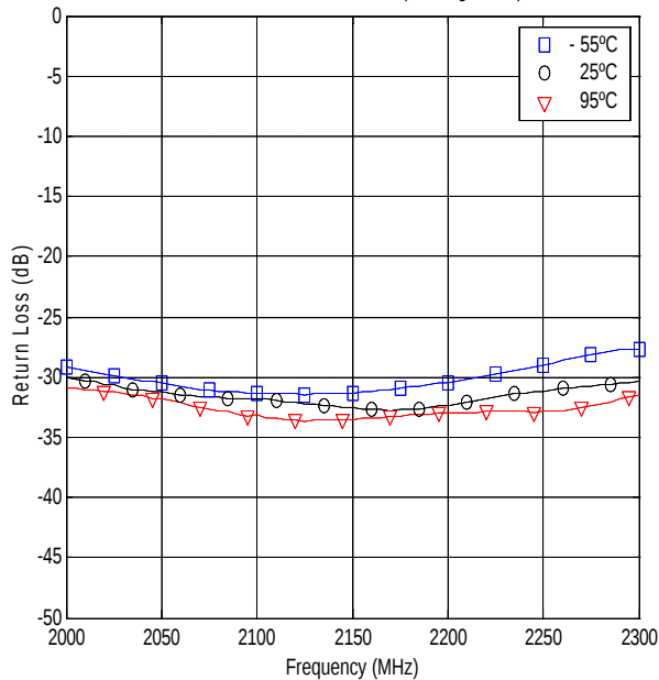
Return Loss for XC2100A-10 (Feeding Port 1)
