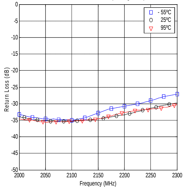
Return Loss for XC2100A-10 (Feeding Port 2)
