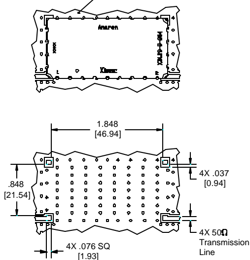
Dimensions are in Inches [Millimeters] XDL09-9-204 Mounting Footprint
