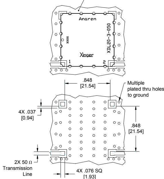
Dimensions are in Inches [Millimeters] XDL20-3-050 Rev A Mounting Footprint
