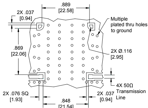
Dimensions are in Inches [Millimeters] XDL 20-7-115 Rev B Mounting Footprint
