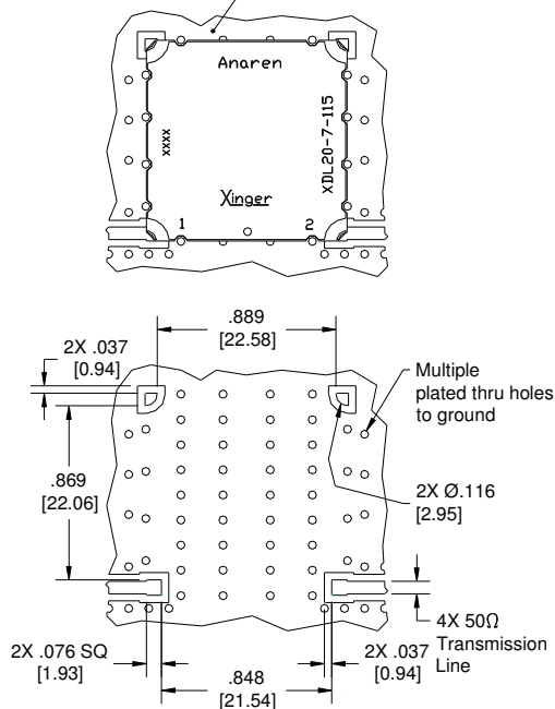
Dimensions are in Inches [Millimeters] XDL20-7-115 Mounting Footprint
