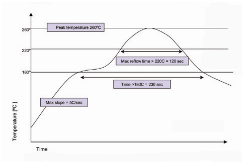
Figure 2 – High Temperature Solder Reflow Thermal Profile
