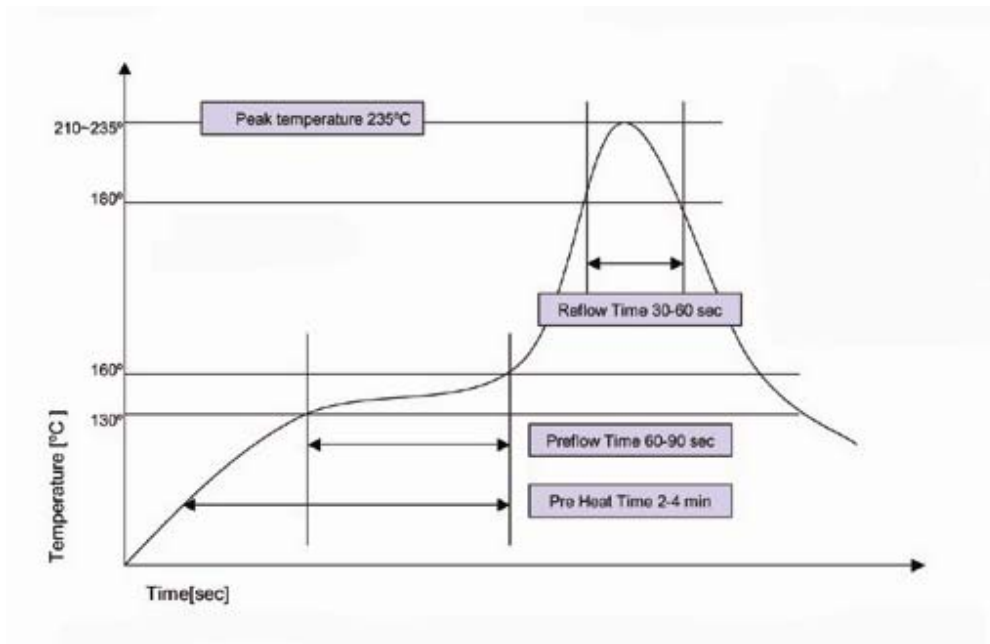
Figure 1 – Low Temperature Solder Reflow Thermal Profile
