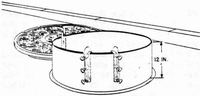
Fig. 3—Adjustable Manhole Shield
