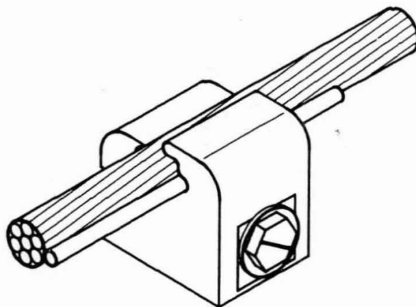
Fig. 2—J Connector—No. 6 Copper Wire to No. 1/0 Ground Wire Connection
