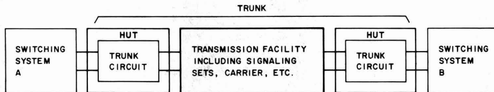
Fig. 9—Relationship of Trunk Circuit to Trunk
