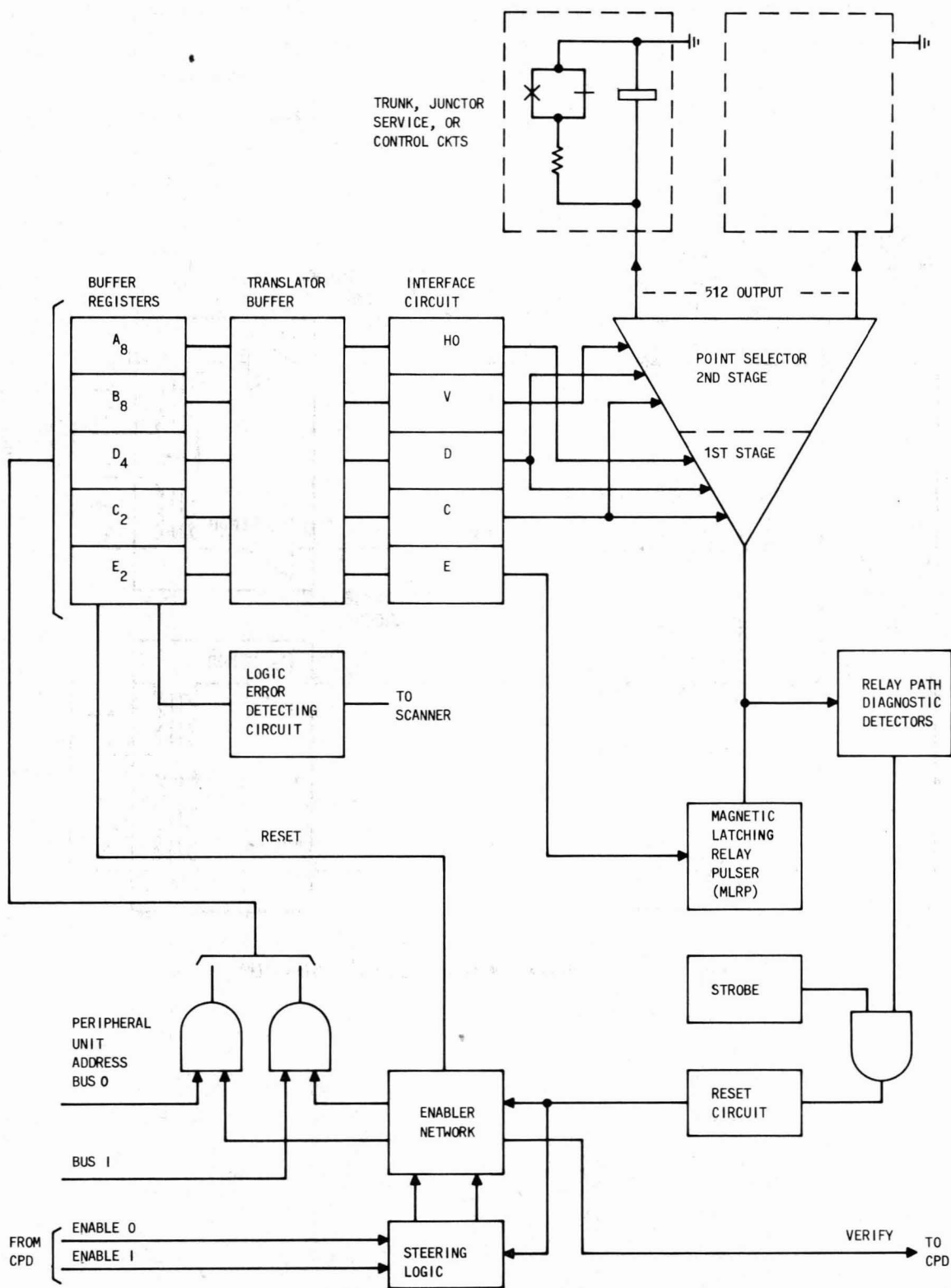
Fig. 12—Basic Signal Distributor Block Controller Diagram
