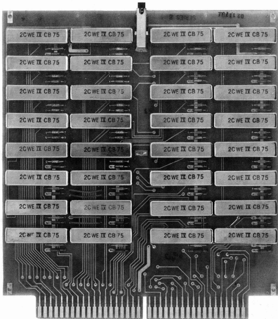
Fig. 7—Plug-in Ferrod Circuit Pack
