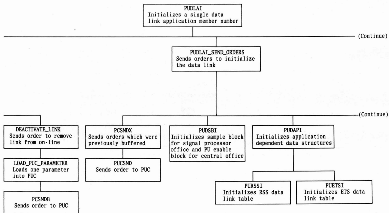
Fig. 11—Subroutine PUDLAI Structural Block Diagram in Pident PUID (Sheet 2 of 3)
