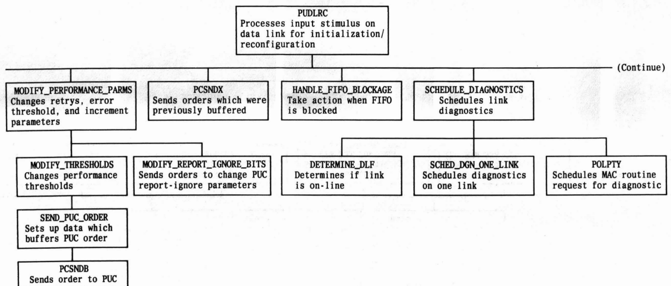
Fig. 9—Subroutine PUDLRC Structural Block Diagram in Pident PUDR (Sheet 3 of 4)
