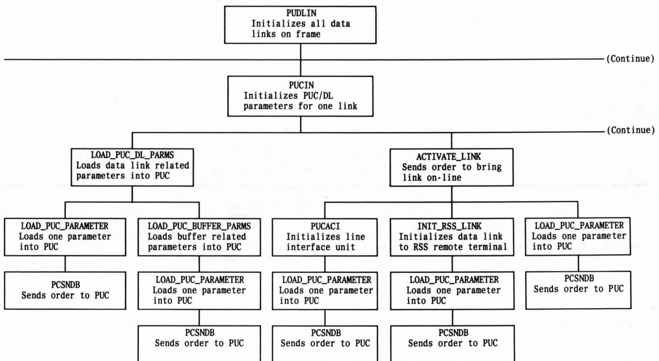
Fig. 10—Subroutine PUDLIN Structural Block Diagram in Pident PUID (Sheet 2 of 3)
