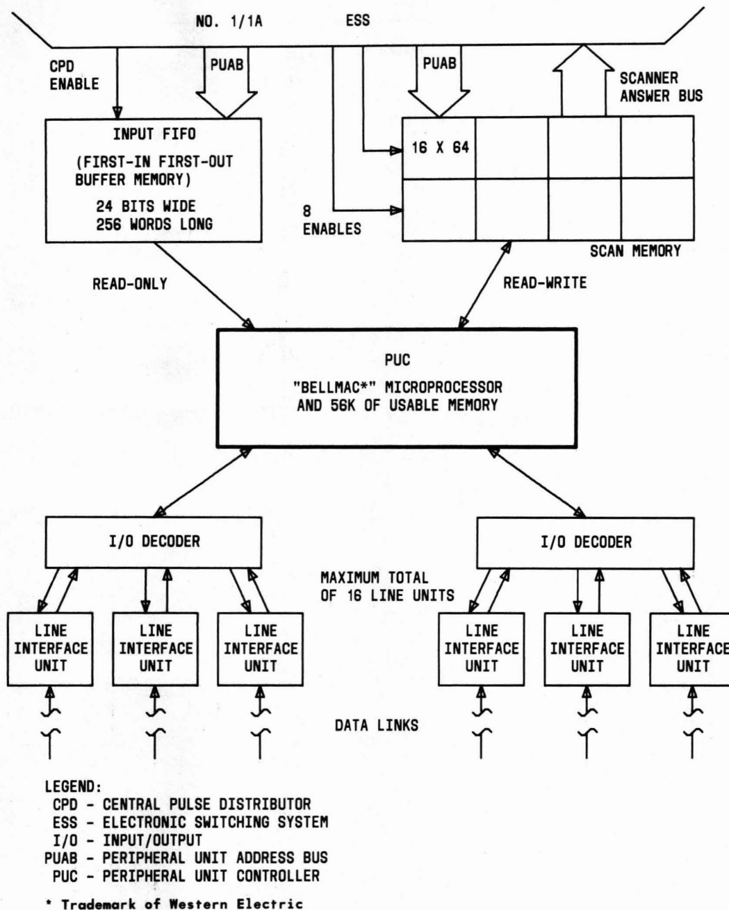
Fig. 5—PUC/DL Processing Units
