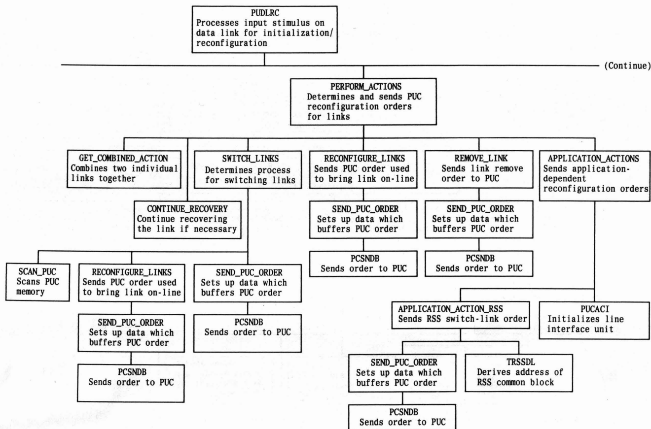
Fig. 9—Subroutine PUDLRC Structural Block Diagram in Pidant PUDR (Sheet 2 of 4)
