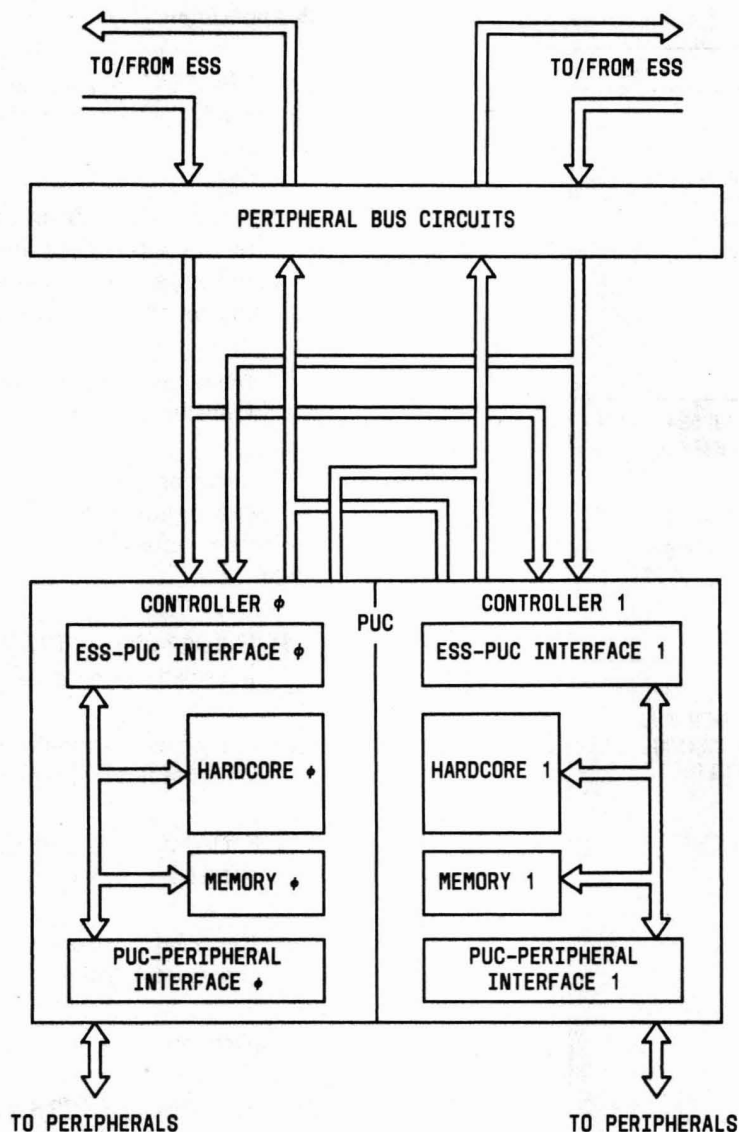
Fig. 2—PUC Block Diagram
