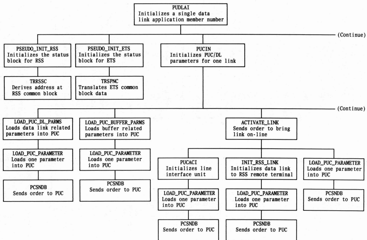
Fig. 11—Subroutine PUDLAI Structural Block Diagram in Pident PUID (Sheet 1 of 3)
