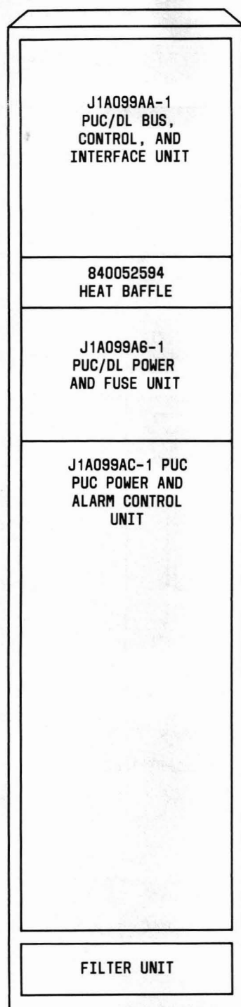
Fig. 1—PUC/DL Frame
