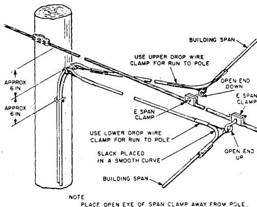
Fig. 22—Spans to Drive Hooks on Pole
