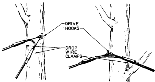
Fig. 15—Turning Corner on Large Diameter Trees
