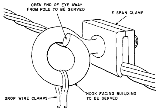
Fig. 21—E Span Clamp Mounted on Strand
