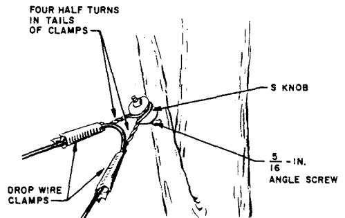
Fig. 17—Turning Corner on Small Diameter Tree
