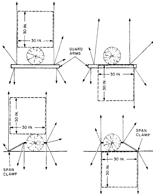
Fig. 2—Drop Wires Distributed From Guard Arm or Span Clamp
