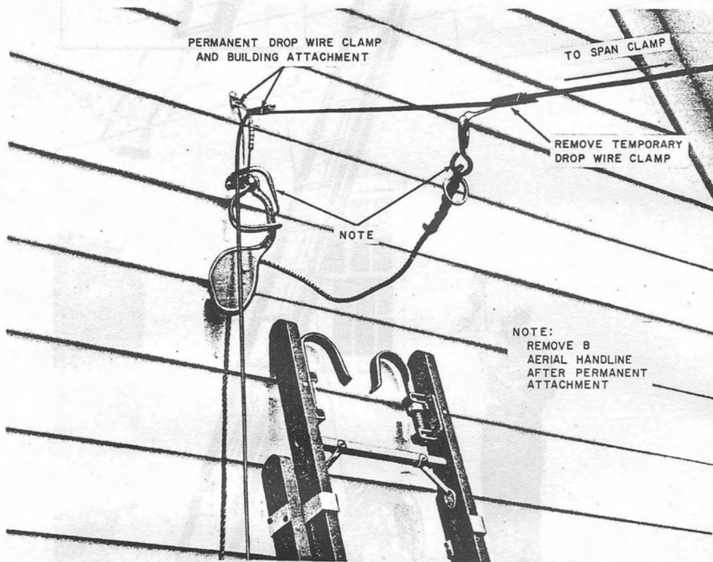
Fig. 32—Completing Permanent Building Attachment
