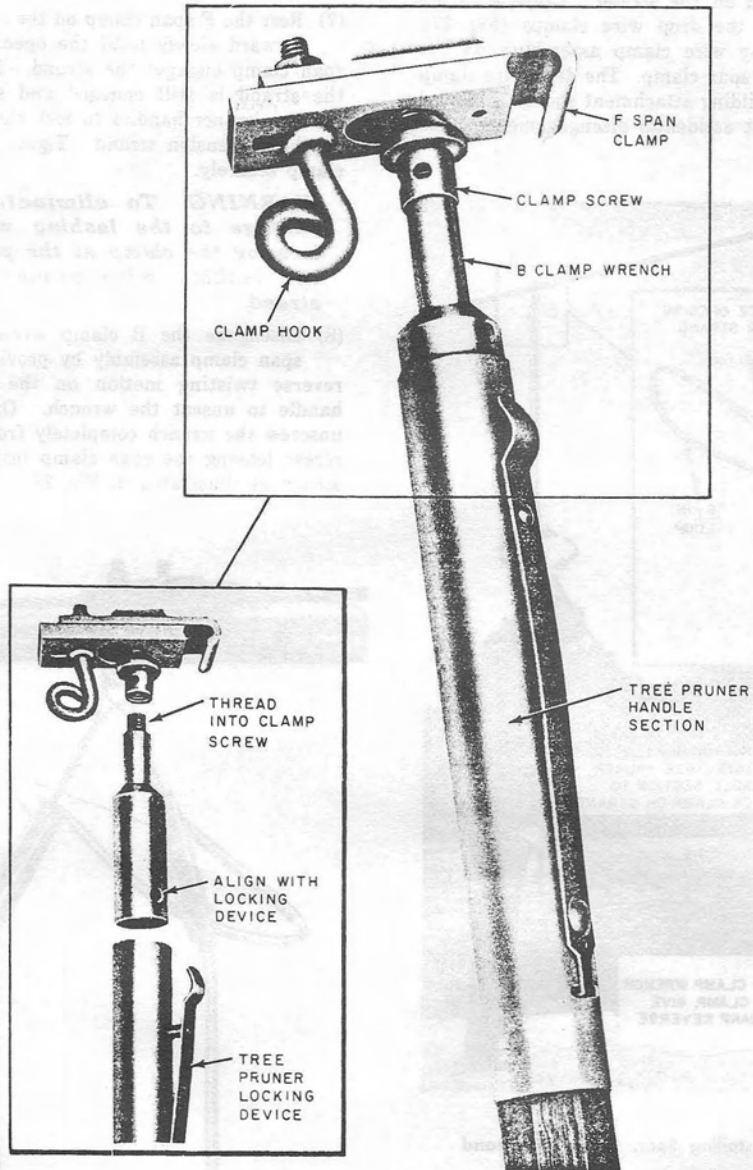
Fig. 26—Clamp and Wrench Attached to Tree Pruner Handle
