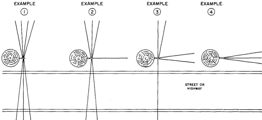
Fig. 4—Maximum Number of Spans Attached to One Drive Hook
