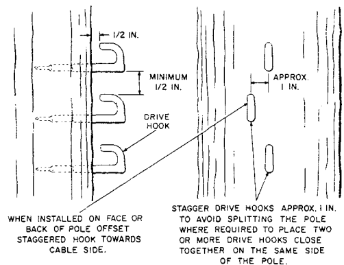
Fig. 3—Drive Hooks Installed in Pole
