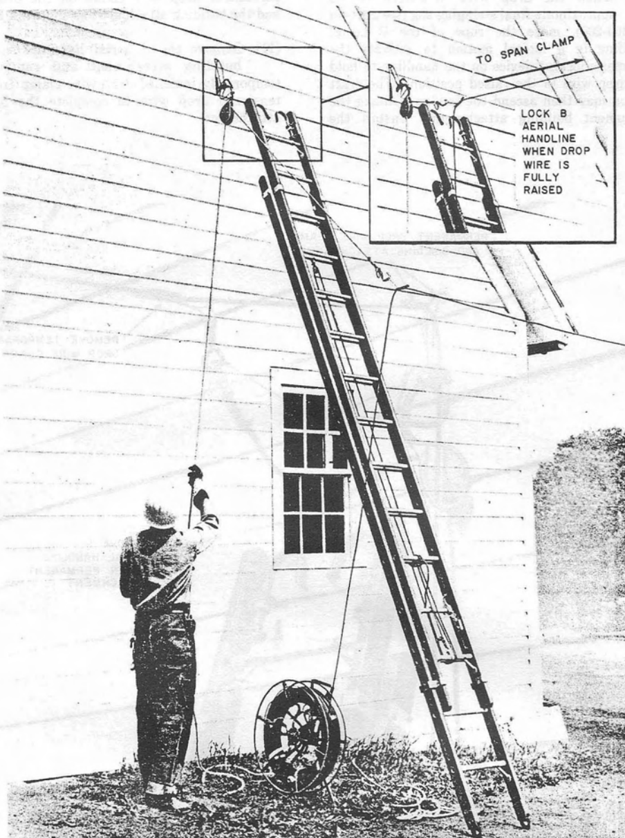
Fig. 31—Raising Drop Wire to Building Attachment
