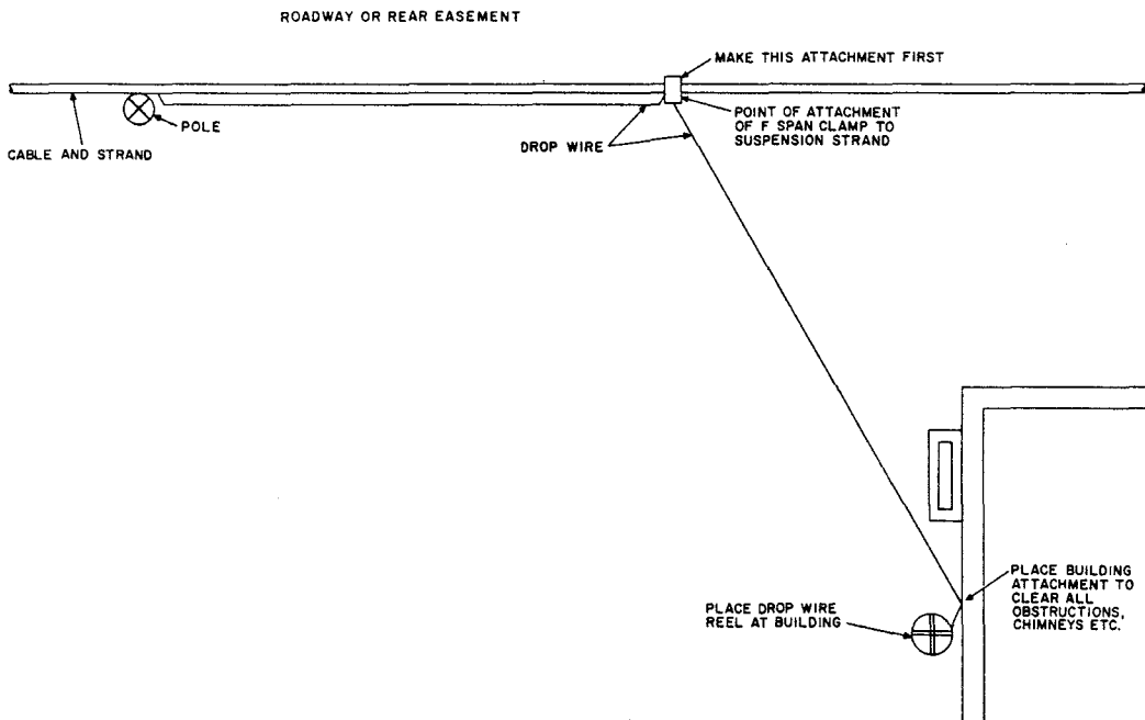
Fig. 25—Relative Positions of Pole, Building, and F Span Clamp
