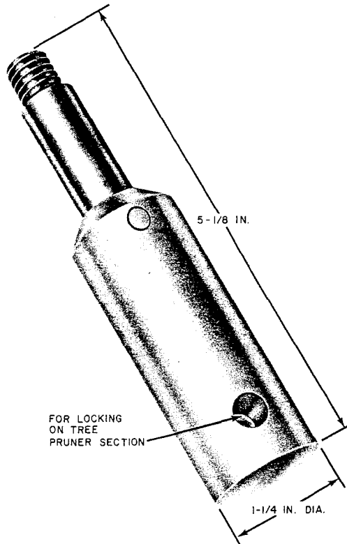
Fig. 24—B Clamp Wrench
