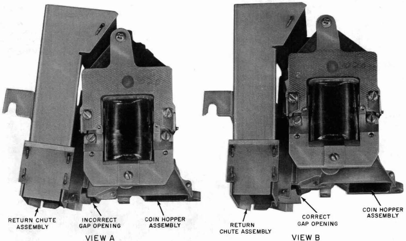
Fig. 8—Alignment of Return Chute Assembly
