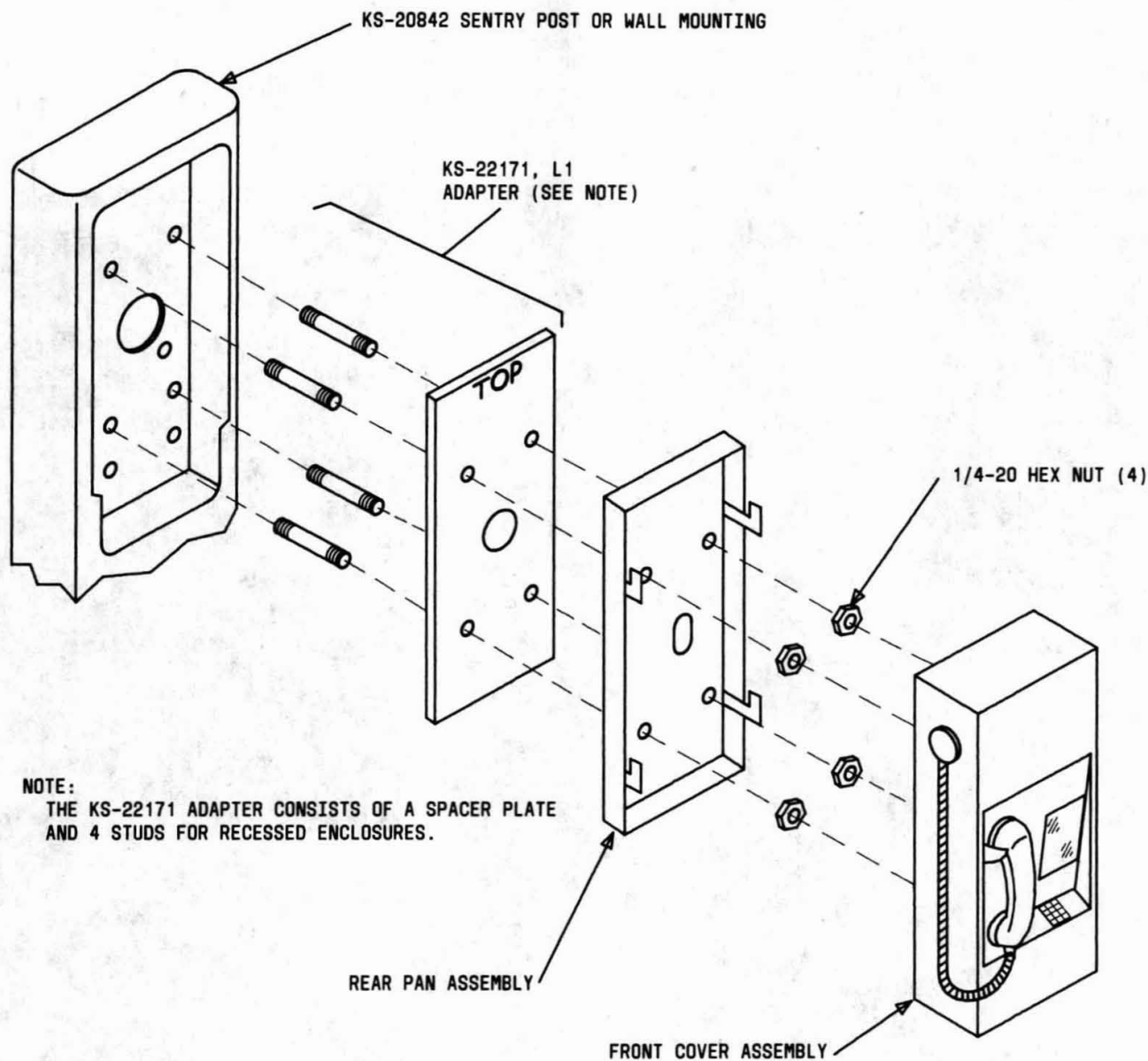
Fig. 6—10A Coinless Telephone Set Used With Adapter
