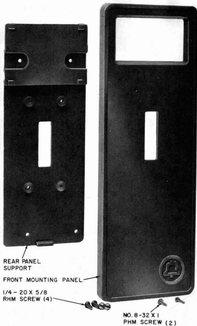
Fig. 9—KS-22284 Backboard
