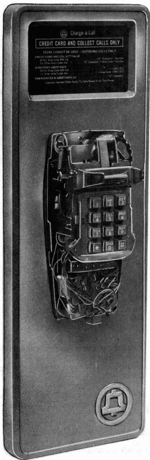
Fig. 13—Installing 2554-Type Telephone Set On Backboard
