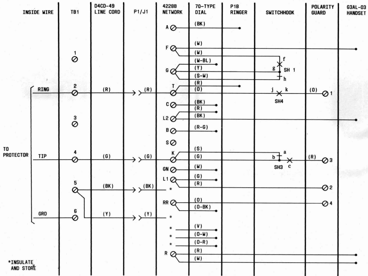
Fig. 17—10A and 20A Coinless Telephone Set, Connections
