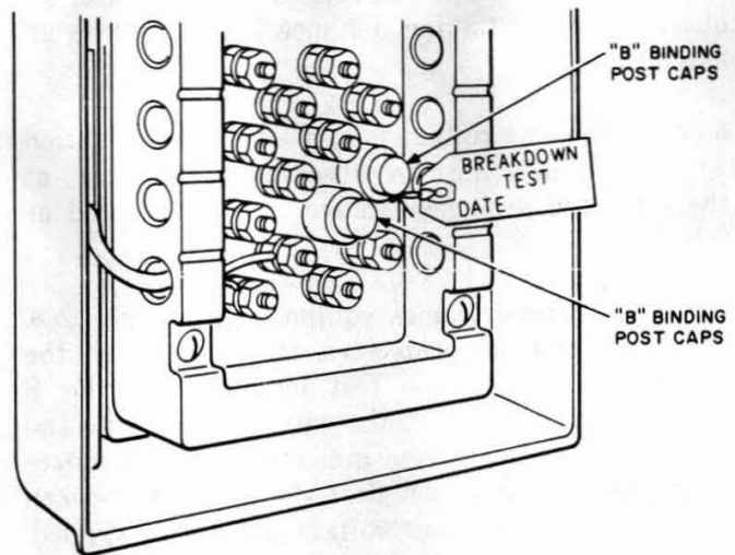
Fig. 14—F-Type Terminal Correctly Protected
