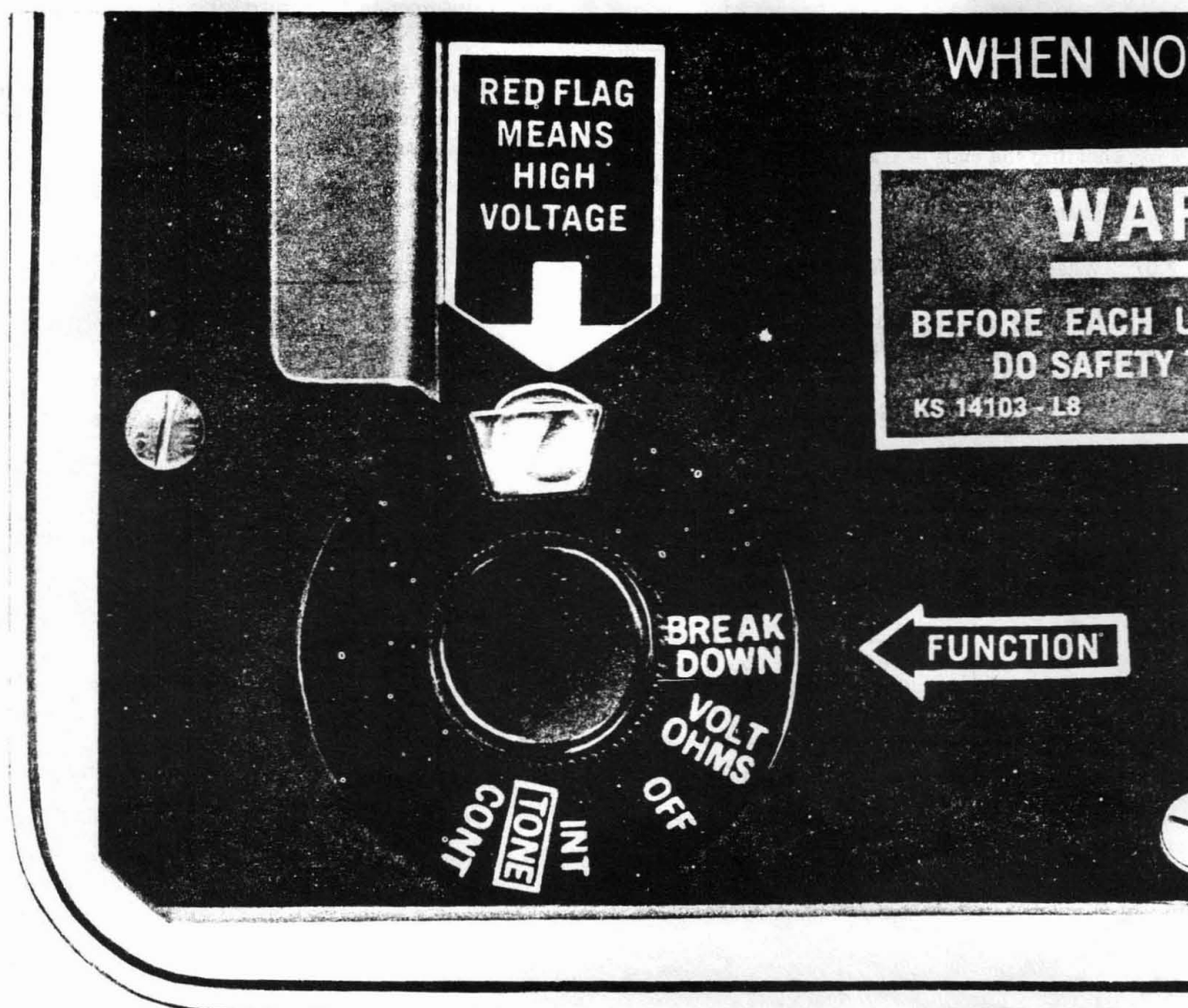
Fig. 16—Indicator Flag On L8 Control Unit
