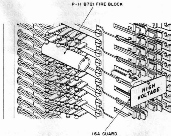
Fig. 10—Protecting B-Type Frames And 444-Type Jacks
