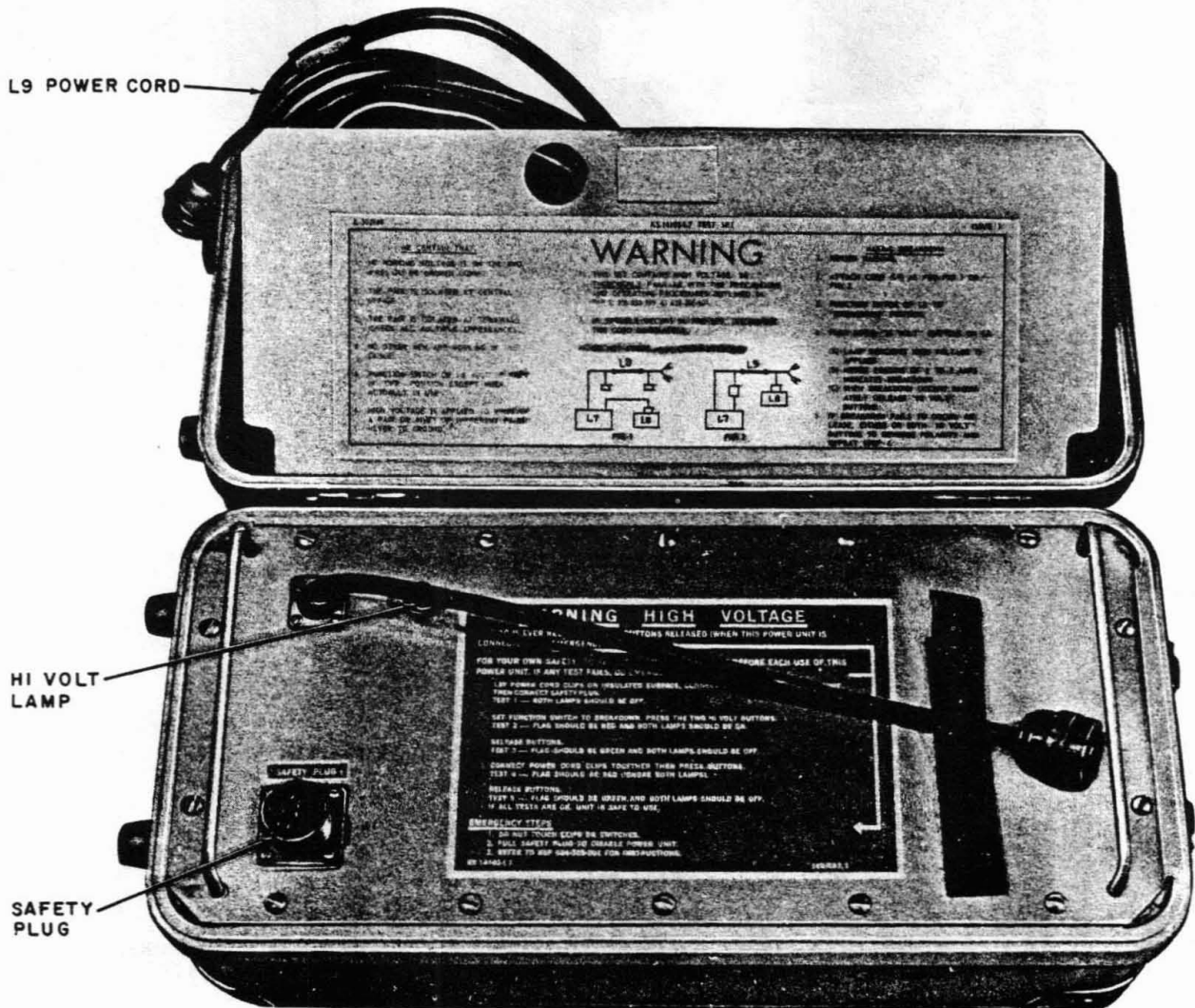
Fig. 1—KS-14103 L7 Power Unit
