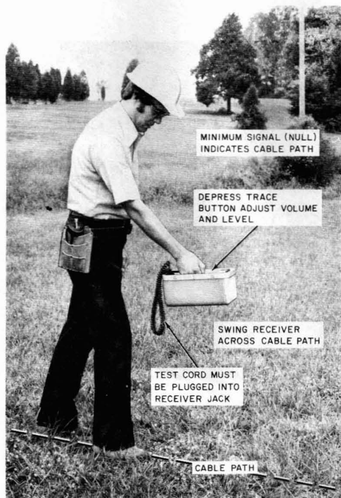
Fig. 14—Tracing Cable Path
