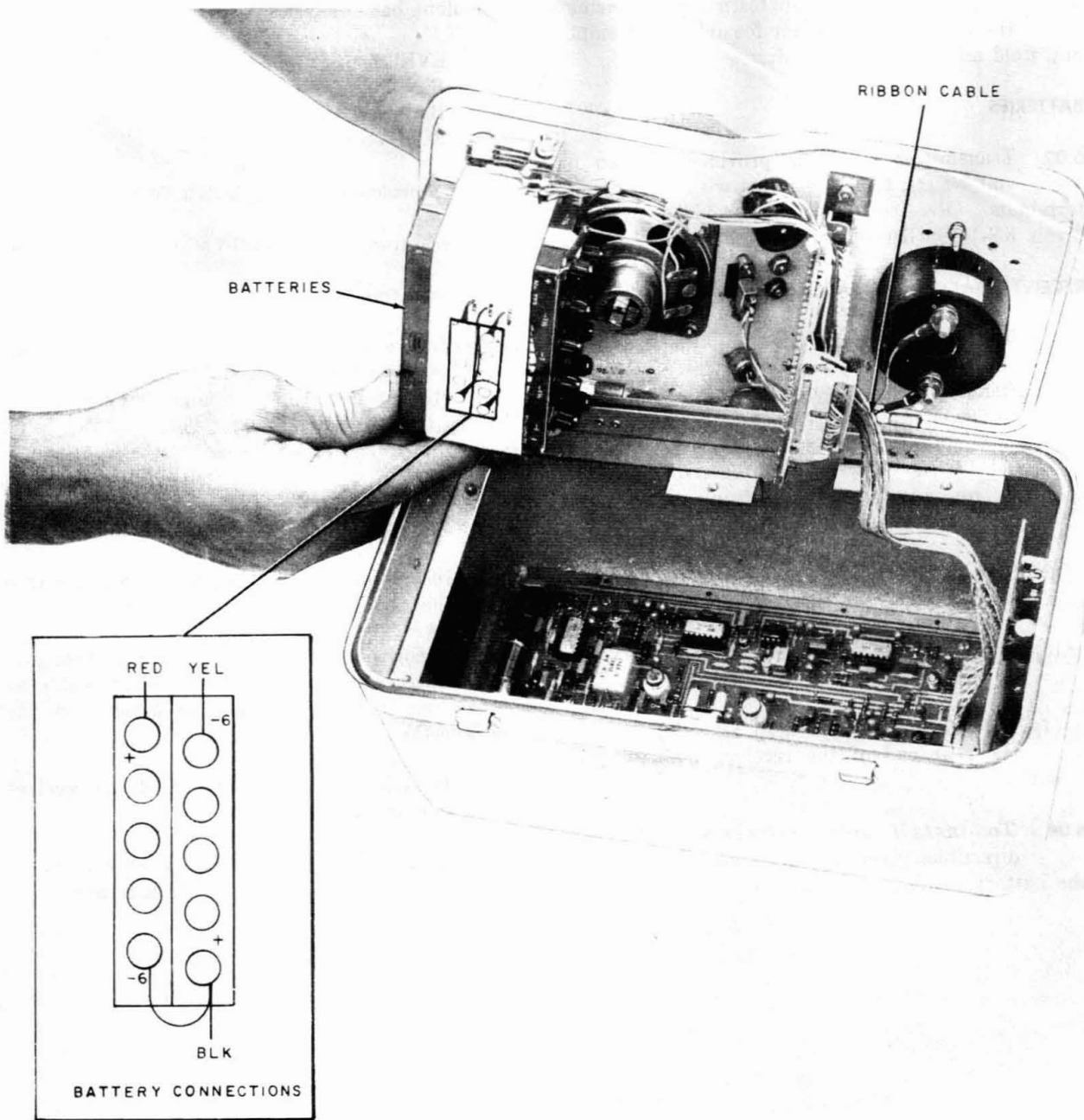
Fig. 16—Receiver Batteries
