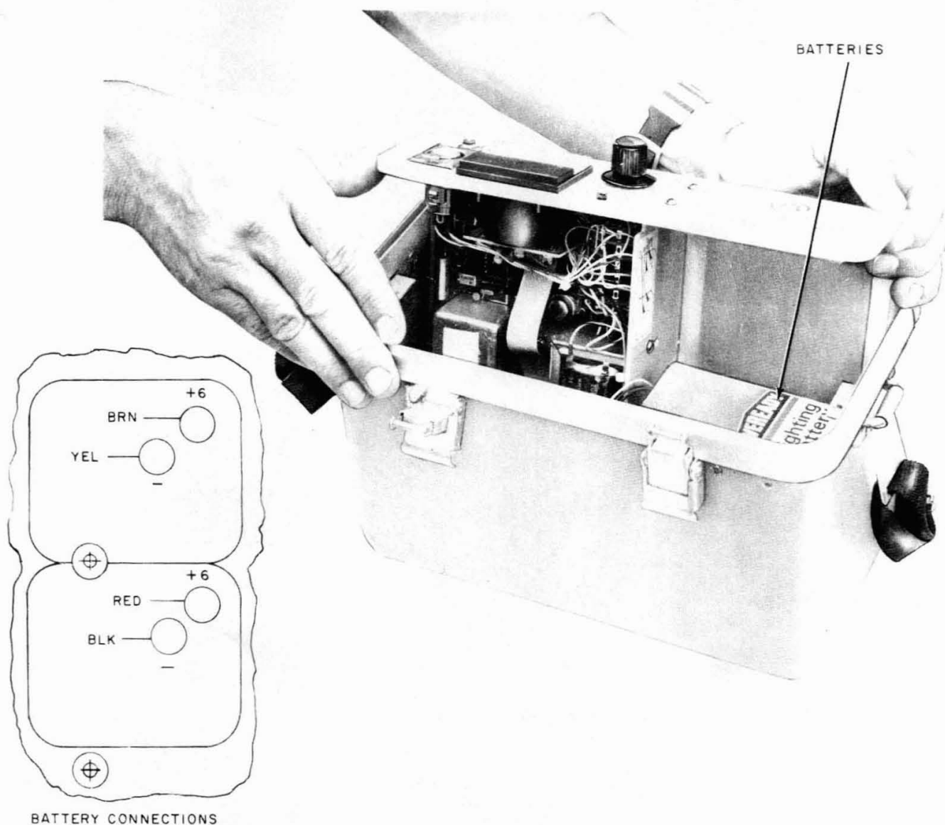
Fig. 17—Transmitter Batteries
