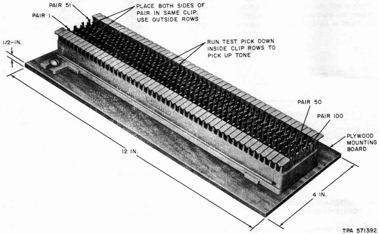
Fig. 6—66M1-50 Connecting Block for Pair Identification
