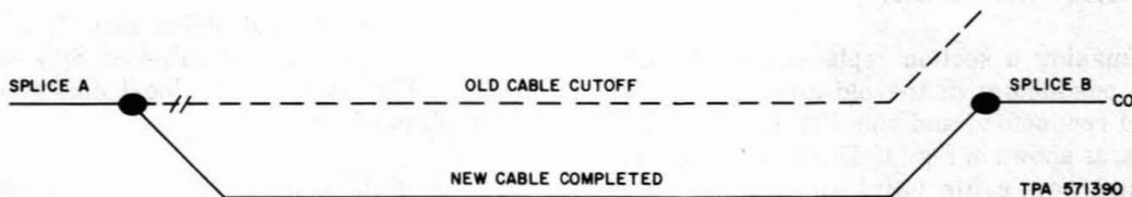
Fig. 4—New Cable Working—Old Cable Cut Off
