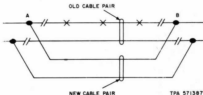
Fig. 1—Section Replacement—Large Cable
