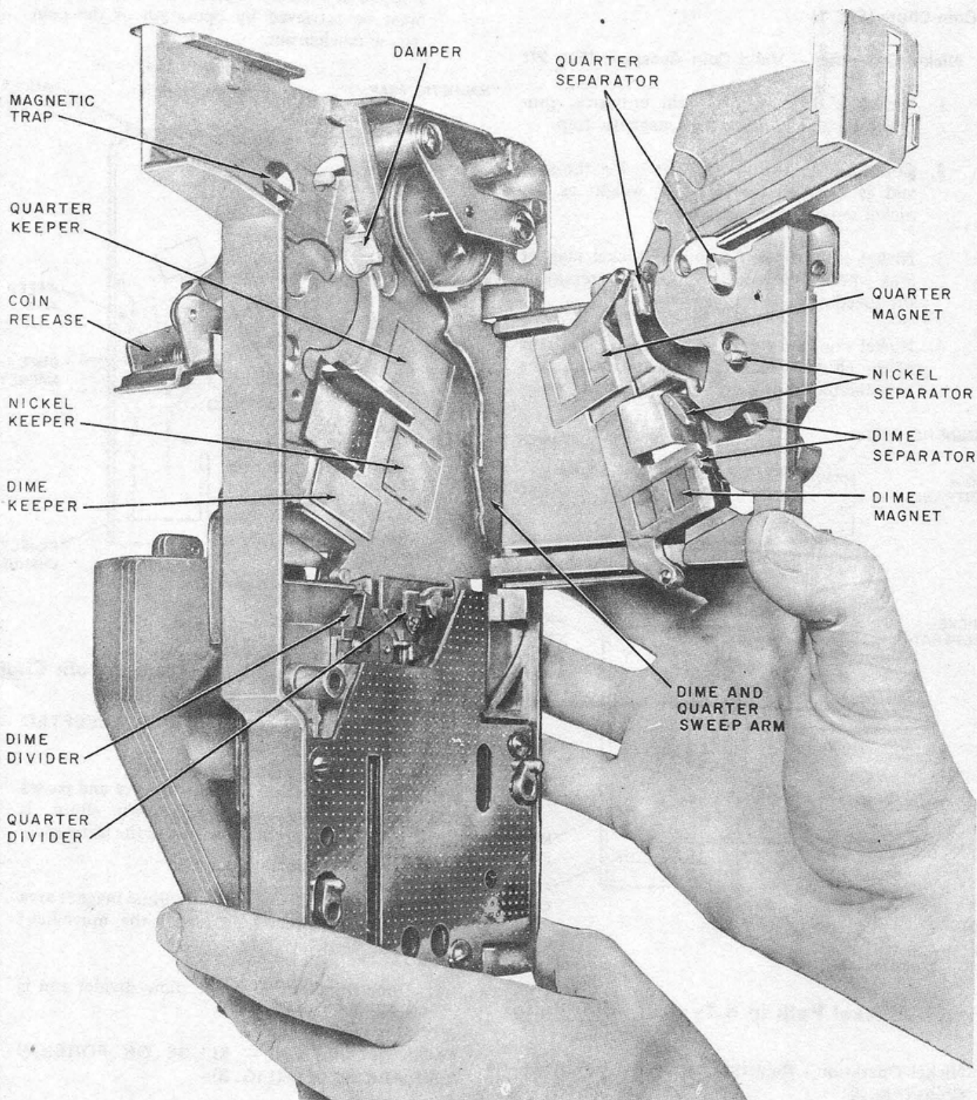
Fig. 1—Typical Coin Chute
