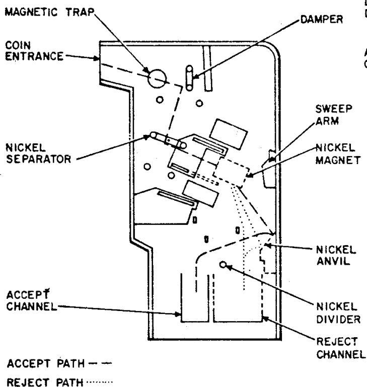
Fig. 2—Nickel Path in a Typical Coin Chute
