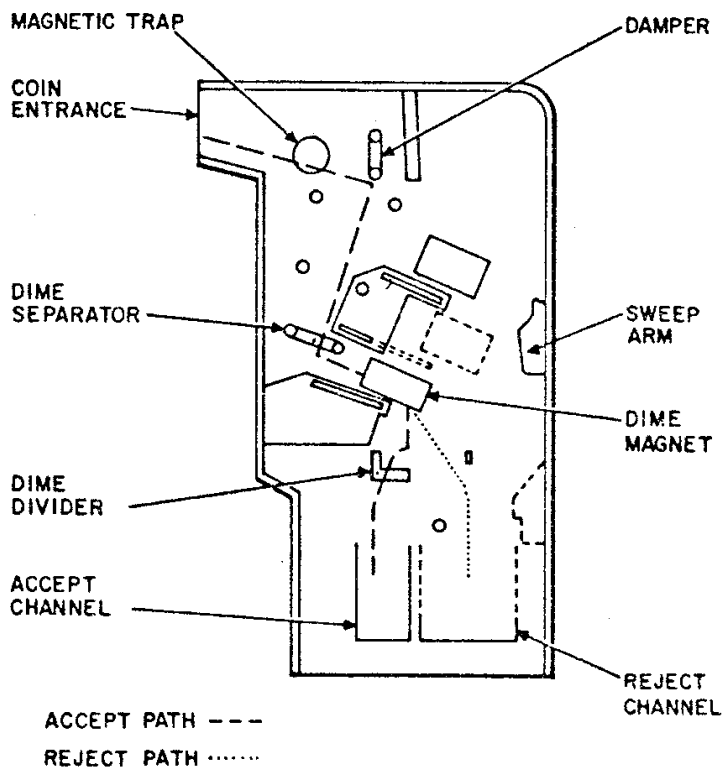
Fig. 3—Dime Path in a Typical Coin Chute
