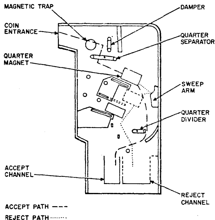
Fig. 4—Quarter Path in a Typical Coin Chute
