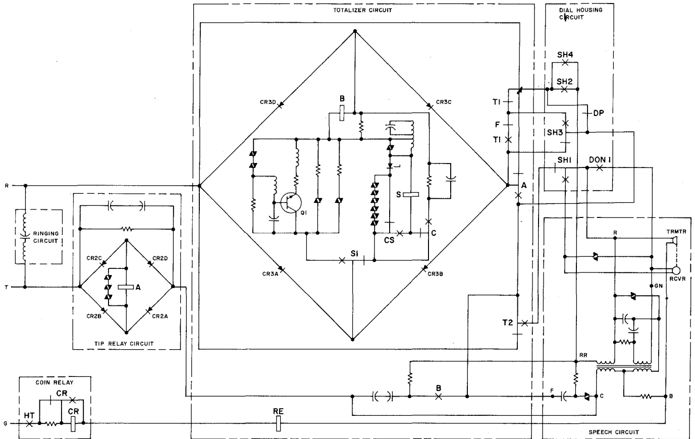
Fig. 11—IC1/2C1 Coin Telephone Set—Schematic (CF Mode)
